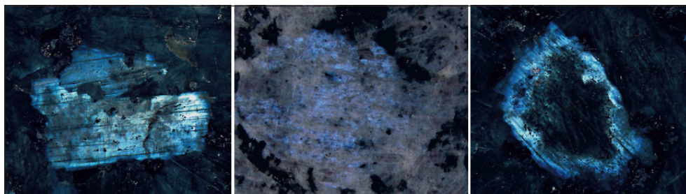
Figure 7. Types of iridescence in feldspar. Left: homogenous. Centre: patchy. Right: zoned. Each photo measures 2 cm horizontally.
