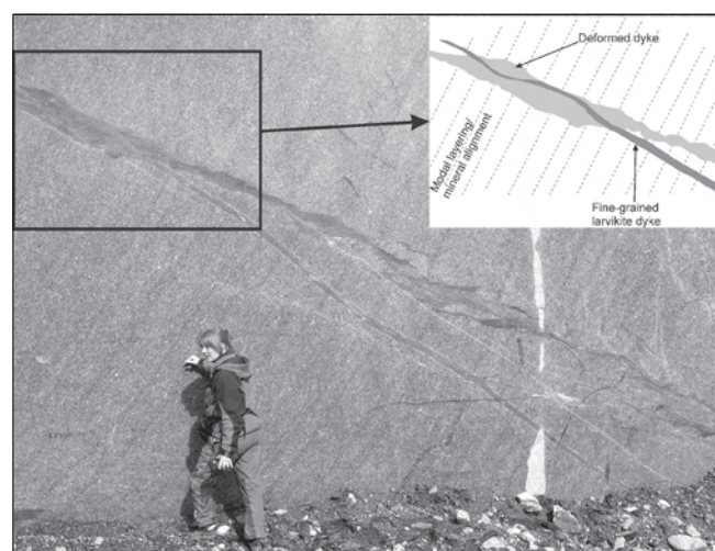
Figure 17. Larvikite dyke cutting shear zone at Malerød. Note mineral alignment and diffuse modal layering (concentration of mafic minerals) in the larvikite.
