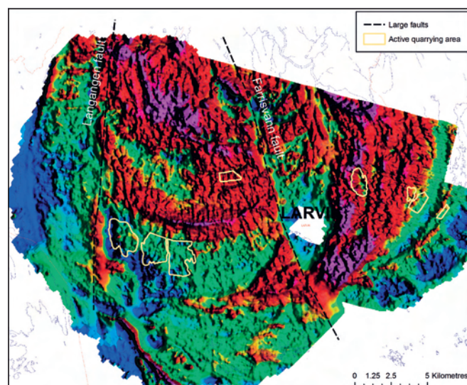
Figure 9. Magnetic anomaly map of the Larvik area, and interpretation of faults.
