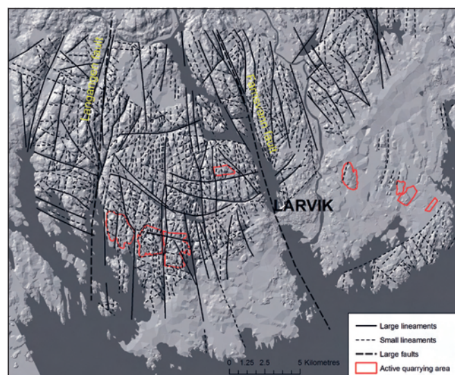
Figure 15. Lineament analysis of the larvikite area.
