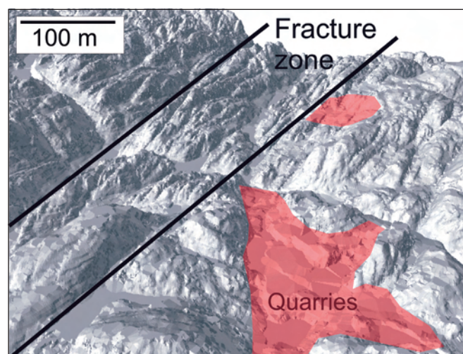
Figure 16. Digital terrain model of the topography in parts of the Tvedalen quarry area, displaying quarries located in a massive part of larvikite beside a large fracture zone.
