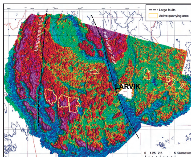
Figure 10. Thorium anomaly map of the Larvik area.
