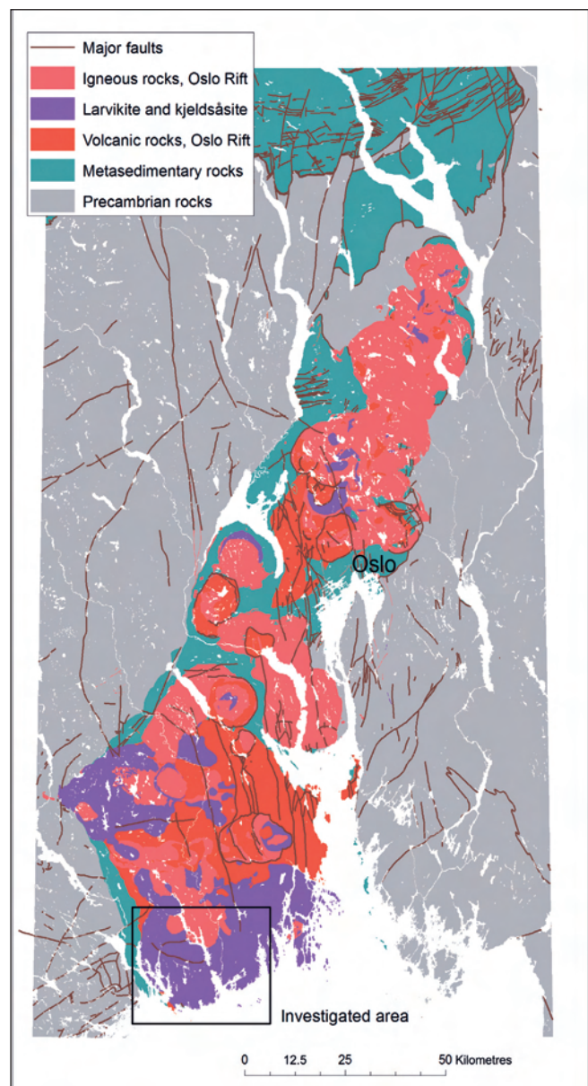
Figure 1. Overview of the Oslo Rift and distribution of larvikite and similar rocks. Modified from NGU digital maps of the Oslo region.
