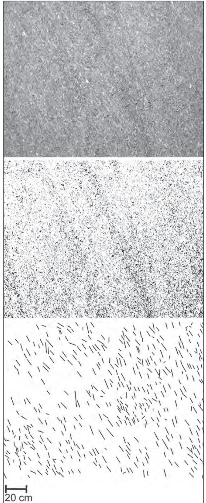
Figure 19 Mineral alignment and modal layering relations. Top: photo of quarry face at Malerød. Middle: distribution of mafic minerals in the same section, displaying diffuse, modal layering. Bottom: feldspar orientation in the same section, being parallel to slightly oblique to the modal layering.
