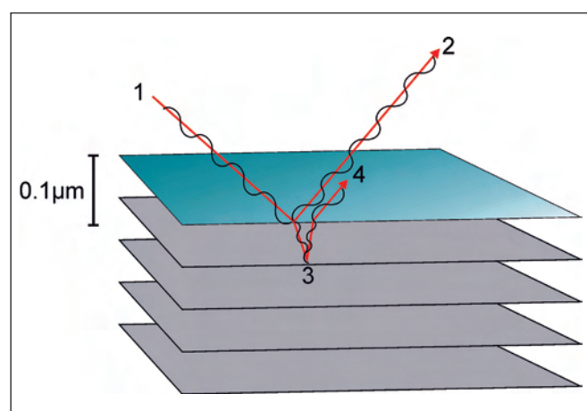
Figure 5. Principle of how iridescence forms in media, such as feldspar crystals. The reflected light beam (1–2) and the refracted beam (1–3–4) reinforce each other because their phase difference is an integral number of wavelengths. Other wavelengths present in a beam incident at this angle will interfere, resulting in the optical interference colours.
