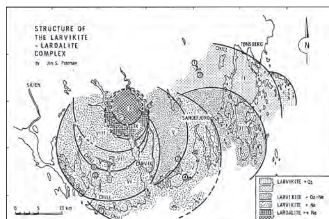
Figure 2. The larvikite ring complex as interpreted by Petersen (1978a). Map from Oftedahl and Petersen (1978).
