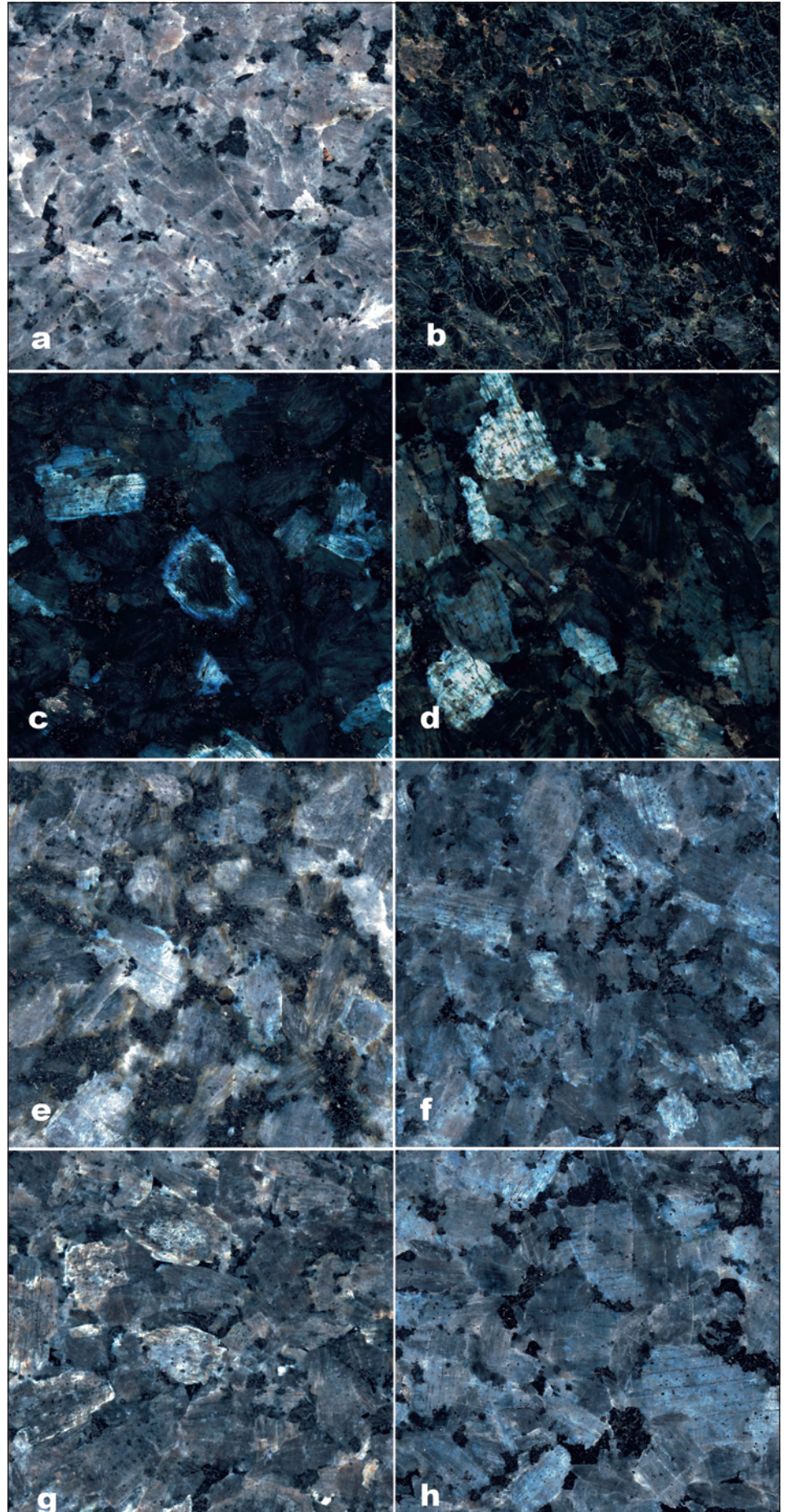
Figure 8. Larvikite subtypes, polished slabs 7 x 7 cm. (a) Kjerringvik, (b) Bergan, (c) Klåstad strong blue (Emerald Pearl), (d) Klåstad silvery to light blue, (e) Stållaker (Marina Pearl), (f) Tvedalen (Blue Pearl), (g) Bassebu, (h) Malerød (Royal Blue).
