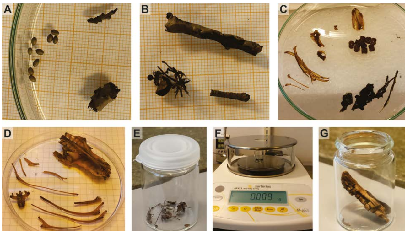
Figure 3.2.9: Some images of hand-picked and cleaned terrestrial plant macrofossils that were radiocarbon dated. A: Nine seeds from a rush plant ( Juncus ), weighing 6 mg; a small willow ( Salix ) twig with buds, weighing 10 mg and a larger birch ( Betula ) twig with attached cortex, weighing 25 mg. These were all found at the isolation boundary in Basin 16 and dated separately; all three yielded identical ages. B: Three other representative dating samples. C: Various remains of a marine fish and some terrestrial leaves and a pine needle (lower right). D: Bones of a long-tailed duck ( Clangula hyemalis ), a rare finding from 11 m depth in the sequence from Basin 4: the pelvis, several ribs and a vertebra. Dated to c. 11 ka. E: A sample of selected plant macrofossils packed in a sterilized vial. F: The same sample being weighed before being submitted to the radiocarbon lab (9 mg – a typical sample size). G: A larger piece of wood ready for dating. Such larger fragments may in theory have remained on the ground for some time after death, prior to deposition in the lake, and may thus pre-date their stratigraphical depth. However, dating of many parallel samples of larger and smaller fragments, both in this and other studies, shows that this is not a significant issue.
