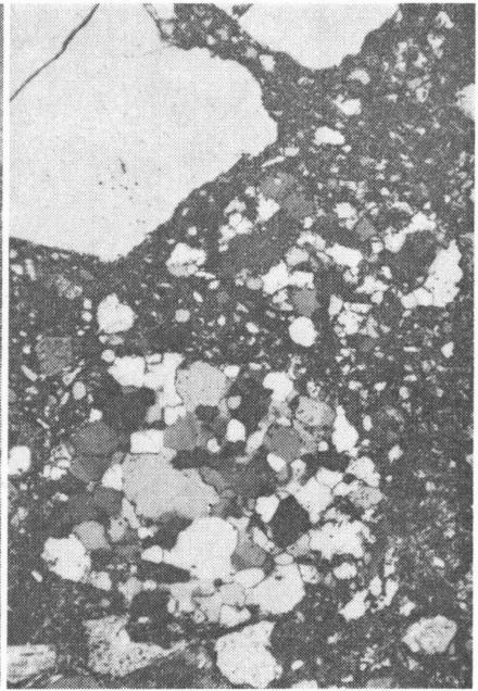
Fig. 5. Microscopic inclusions of rounded quartzitic rocks. Crossed nicols. x 40 magnification.
