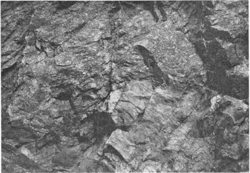
Fig. 6. Sharp contact between the tuffisite and the adjacent gneissose rocks. Roadcut Hjølmodalen.
