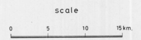
Fig. 2 MAP OF METAMORPHIC FACIES DISTRIBUTION WITHIN SOUTHERN TROMS AND THE NORTHERN PART OF THE OFOTEN AREA
