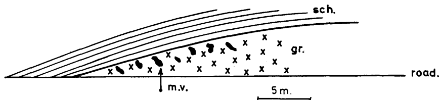
Fig. 6. Microcline veins (m.v.) in Rombak granite (gr.) near the boundary against the Rombak Group (sch.). Skjomen.
