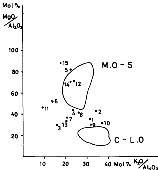
Fig. 33. Plotting of analyses on a diagram after K. Bjørlykke (1965). C - L.O. = Cambrian and Lower Ordovician of the Oslo area and Sweden. M.O. - S = Middle Ordovician and Silurian of the same areas.
