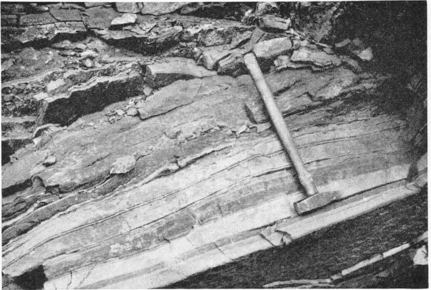
Fig. 27. Alternating layers of plagioclase gneiss and mica schist, Narvik Group, Løkse, Salangen.
