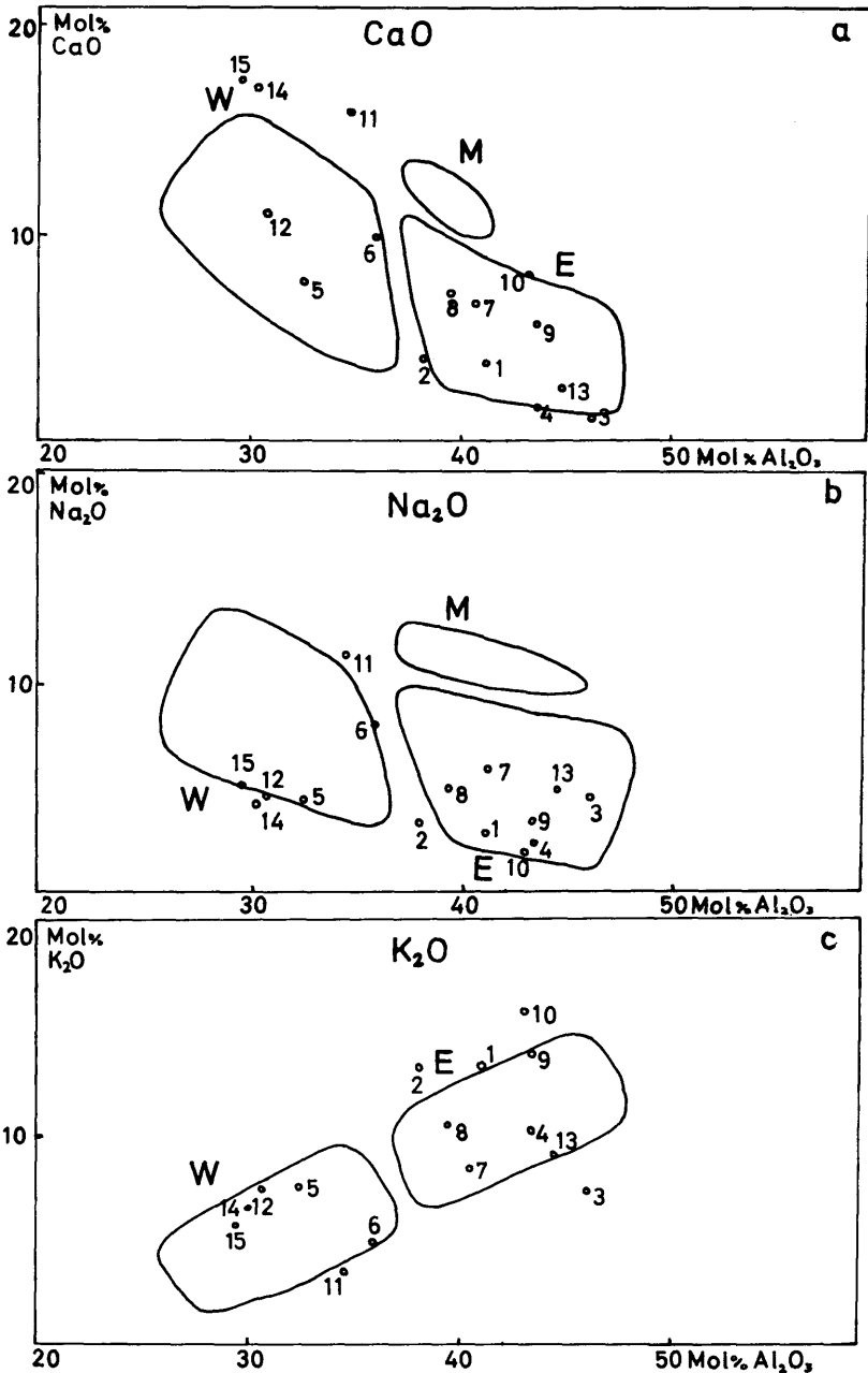
Figs. 32 a—e. Plotting of chemical analyses from the area on the diagrams of Vogt.
