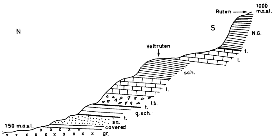
Fig. 23. Section through Hyolithes Zone, Storjfjell Group, Rombak Group and the lowest part of the Narvik Group on the northern slopes of Ruten, Målselv. (gr. = Precambrian granite, sa. = Hyolithes sandstone, q.sch. = quartz schist of the Storjfjell Group, l. and sch. = meta-limestones and mica schists of the Rombak Group, N.Gr. = Narvik Group, t = thrust planes.)
