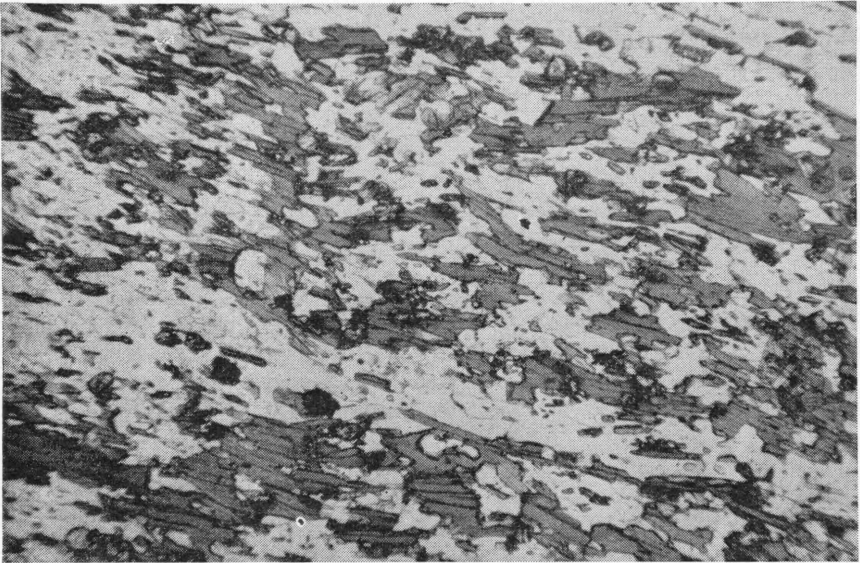
Fig. 34. Typical Rombak schist, 3.4 km E. of Trelidal showing pronounced parallel texture due to orientation of biotite, epidote and quartz aggregates (35x).
