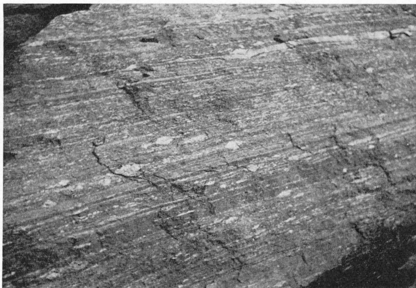
Fig. 28. Gneiss with augens of plagioclase, Narvik Group. Compositional banding is visible. Height of picture about 2 m.
