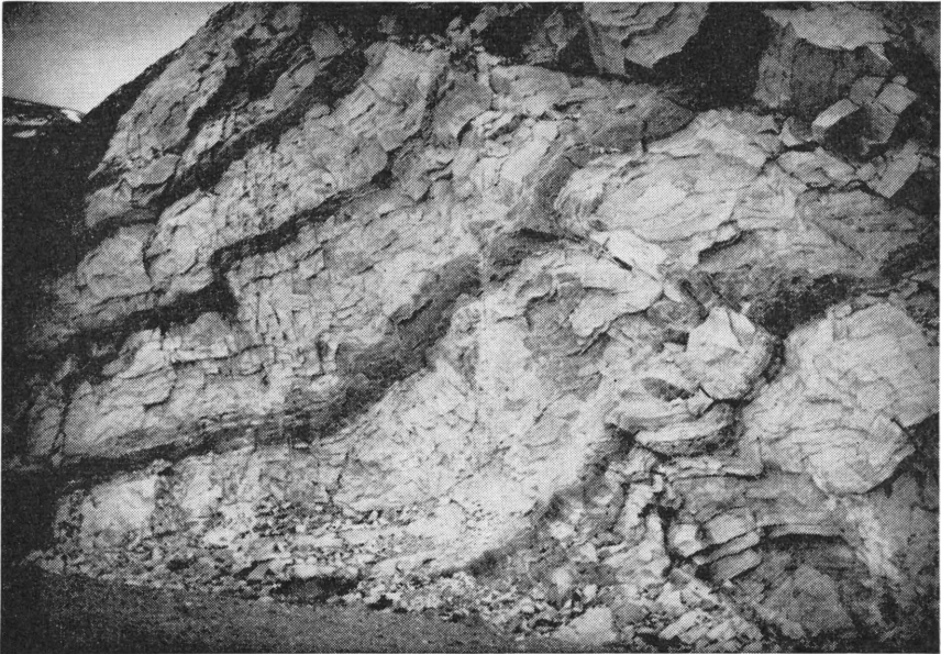
Fig. 25. Sjøvegan quartzite with pelitic intercalations, Narvik Group. Rotvik, Salangen.
