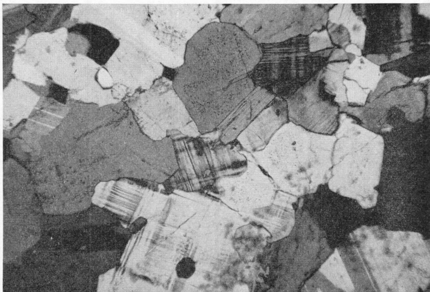
Fig. 10. Normal Tysfjord granite, Æfjord. The minerals are microcline, plagioclase, quartz and biotite (+n., 35x).
