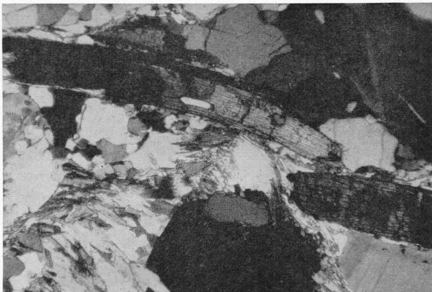
Fig. 38. Kyanite and garnet in plagioclase gneiss, Lemman, Skjomen. One of the kyanites is bent and is showing uneven extinction. The kyanite prisms are parallel or sub-parallel to the foliation (+n. 35x).
