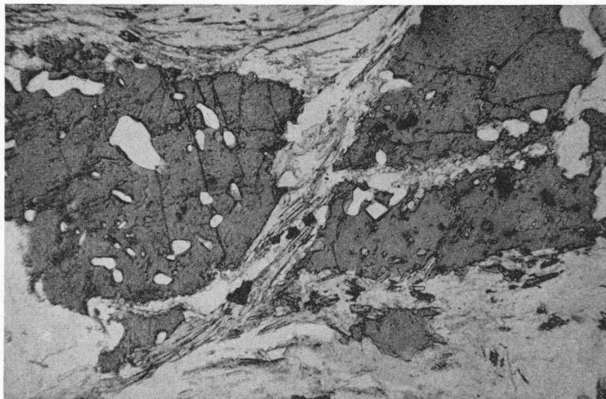
Fig. 37. Amphibole porphyroblasts in Seternes schist broken by late tectonic movements. Crackfillings of chlorite + quartz (35x).
