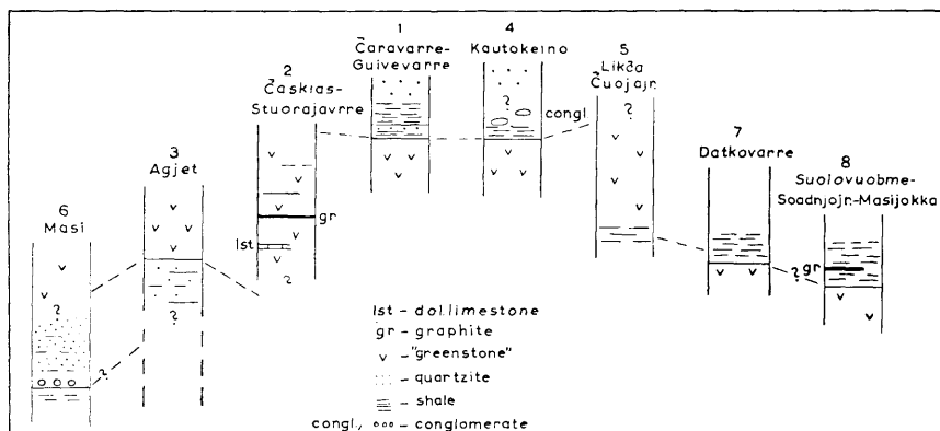
Fig. 8. Diagram to show the suggested correlation of the main formational units. Not to scale.
