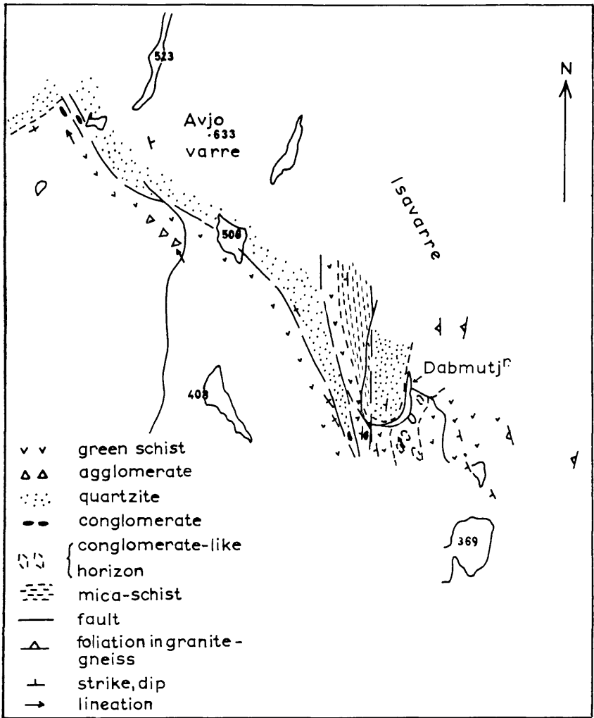
Fig. 18. Geological map of the Dabmutjavre region.
