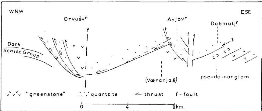
Fig. 19. Diagrammatic section between Orvušvarre and Dabmutjavrre to show the suggested relationships. Vertical scale much exaggerated.
