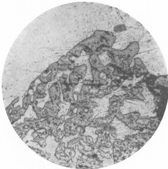
Phot. 11. Native silver (white) replaces marcasite partly rendered to pyrite (grey). 300 \times . Mine Kongens grube. 520 m level.
