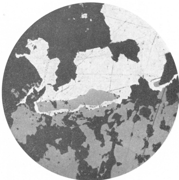
Phot. 6. Young sphalerite (grey) replaces native silver (white) within a coating of chloantite (light grey). Calcite (black). 100 \times . Mine Haus Sachsen. 480 m level.
