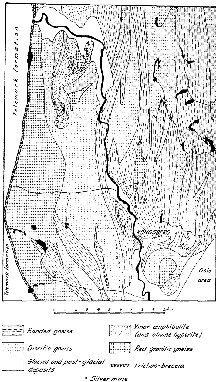
Fig. 3. Geologic map of Kongsberg mining district. Reconstructed after A. Bugge and C. Bugge.
