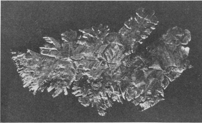
Fig. 13. Lamini-formed crystal of native silver.
