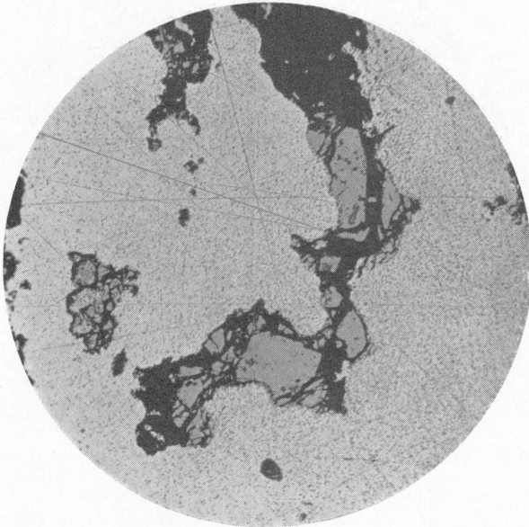
Phot. 4. Veinlet of calcite (black), niccolite (dark grey) and chloantite (light grey) in native silver (white, tarnished). Same paragenesis as Phot. 3, but without pyrrhotite and chalcopyrite. 50 ×. Mine Gottes Hülfe in der Noth.
