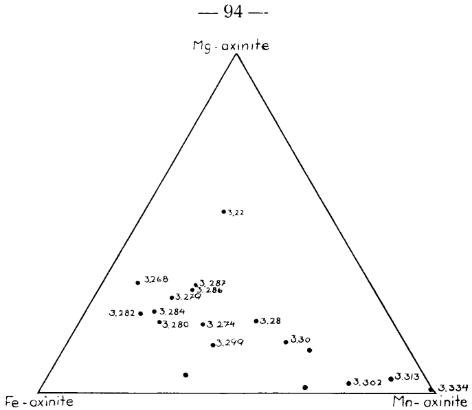
Fig. 34. Diagram showing chemical composition of axinites and corresponding specific gravities.
