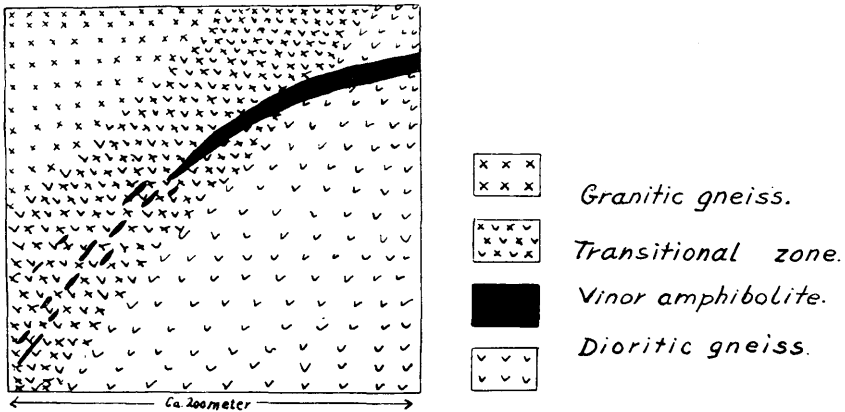
Fig. 4. Boundary between granitic gneiss and and dioritic gneiss. SE Skriverplass, Gomsrud. After C. Bugge. Author's nomenclature.
