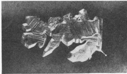
Fig. 14. Small lamini-formed crystal of native silver.
