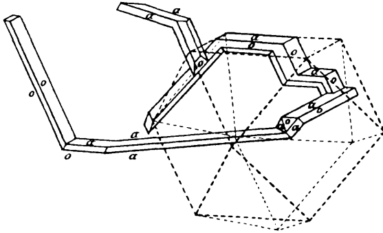
Fig. 11. Twin crystals of silver. a = cube. o = octahedron. After A. Sadebeck (60).
