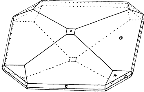
Fig. 24. Crystal of anatase. o (017), r (115), p (111), e (101), c (001).
