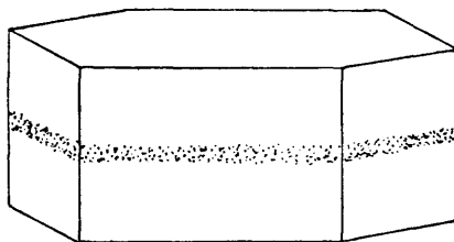
Fig. 21. A crystal of calcite pigmented with pyrrargyrite in a zone parallel to the base.
