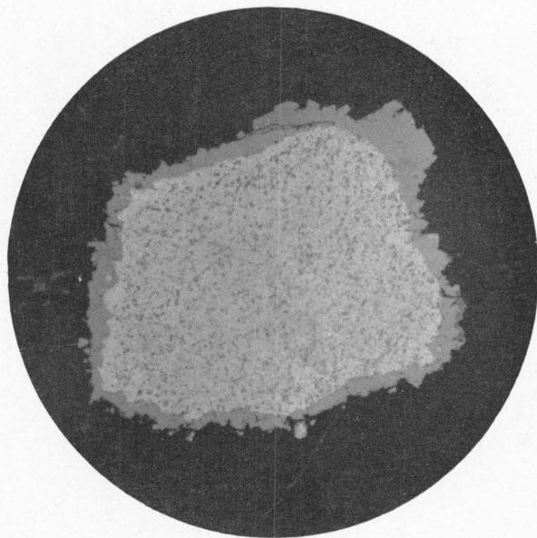
Phot. 16. Coating of rammelsbergite (grey) around a thread of native silver (white, tarnished). Calcite (black). 300 \times . Mine Cristian VII. 150 m level.
