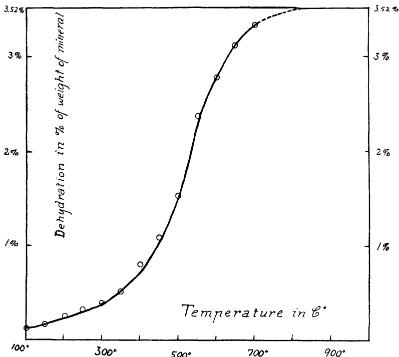
Fig. 37. Dehydration curve of armenite.
