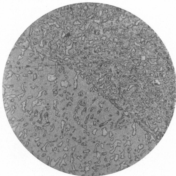
Phot. 12. Native silver (white) replaces marcasite which is partly rendered to pyrite (grey). Note border between twin crystals of marcasite. 200 \times . Mine Kongens grube. 520 m level.
