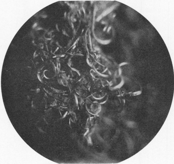
Fig. 5. Malachite in threads as pseudomorphs after native copper. From a sulphide-bearing quartz - breccia vein in Lassedalen.
