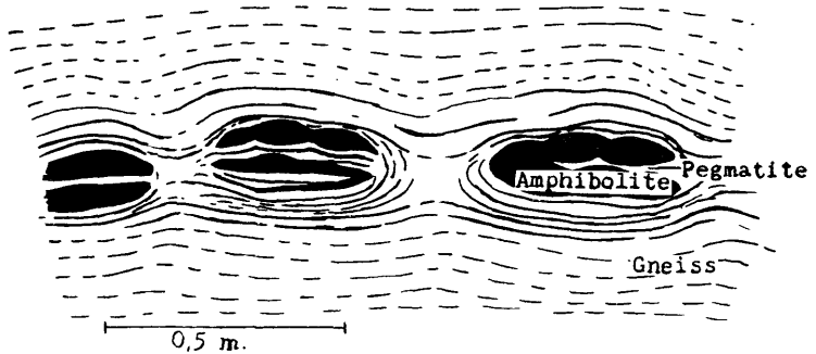
Fig. 9. Boudinage in banded gneiss.
