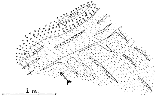
Fig. 4. Boundary between granite and gneiss, in the apex of the angle between the main granite body and the appendix in the southwestern part of the granite area. Here, too, the foliation of the granite follows the boundaries. The gneiss, being strongly folded with the folding axes dipping under the granite, is dissected by small pegmatite veins at the boundary. Only in a narrow zone along the boundary itself the schistosity of the gneiss is conformable to it, as a result of the contact. Here, the granite sends small apophyses along the schistosity planes, and partly includes gneiss, whose schistosity is then conformable to the foliation of the granite.
