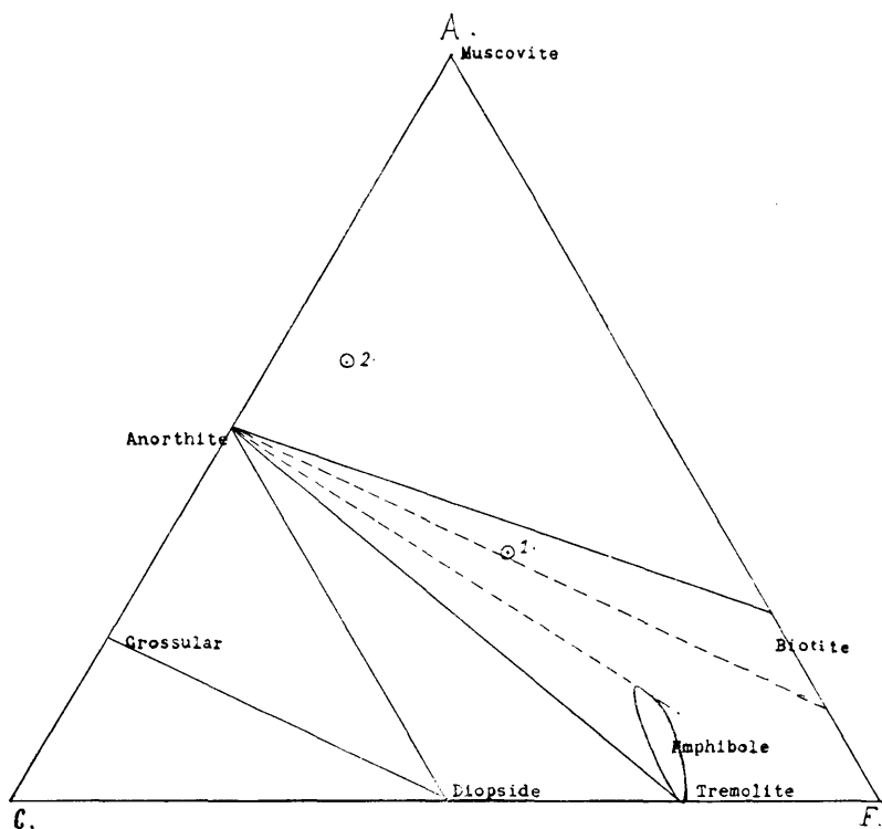
Fig. 3. ACF-diagram for amphibolite-facies. 1. Levang granite. 2. Gneiss.
