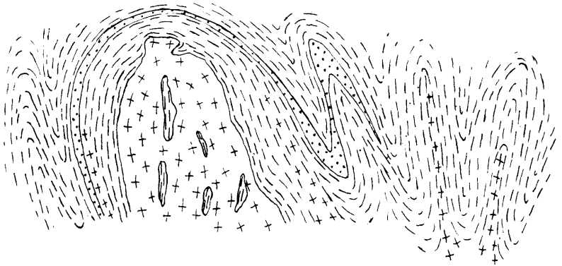
Fig. 16. Vertical section through the Levang granite.
