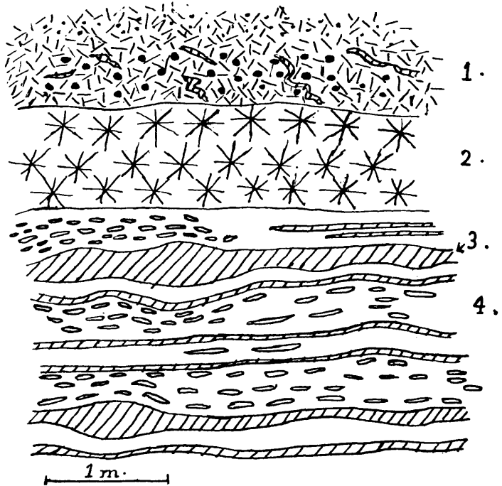
Fig. 11. Anthophyllite- and sillimanite-bearing gneiss on the southern shore of Tåtøy. 1. Amphibolite with garnet porphyroblasts and pegmatite veins. 2. Anthophyllite crystals. 3. Pegmatite. 4. Gneiss with sillimanite nodules.
