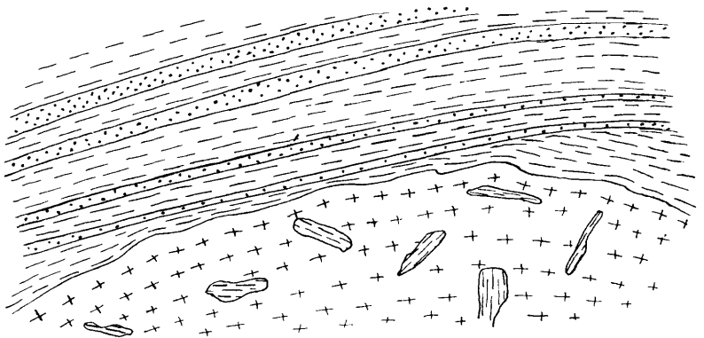
Fig. 17. Vertical section through the Levang granite.
