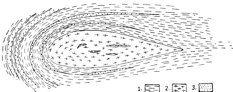
Fig. 15. Section through the Levang granite, parallel to the surface. 1. Gneiss. 2. Granite. 3. Quartzite.
