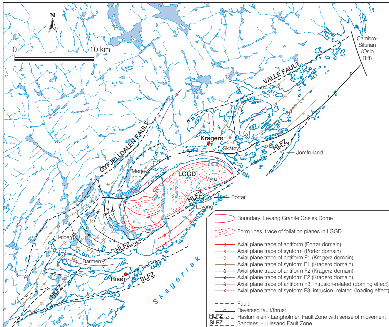
Fig 10. Map showing the main structural elements present in the area of study.
