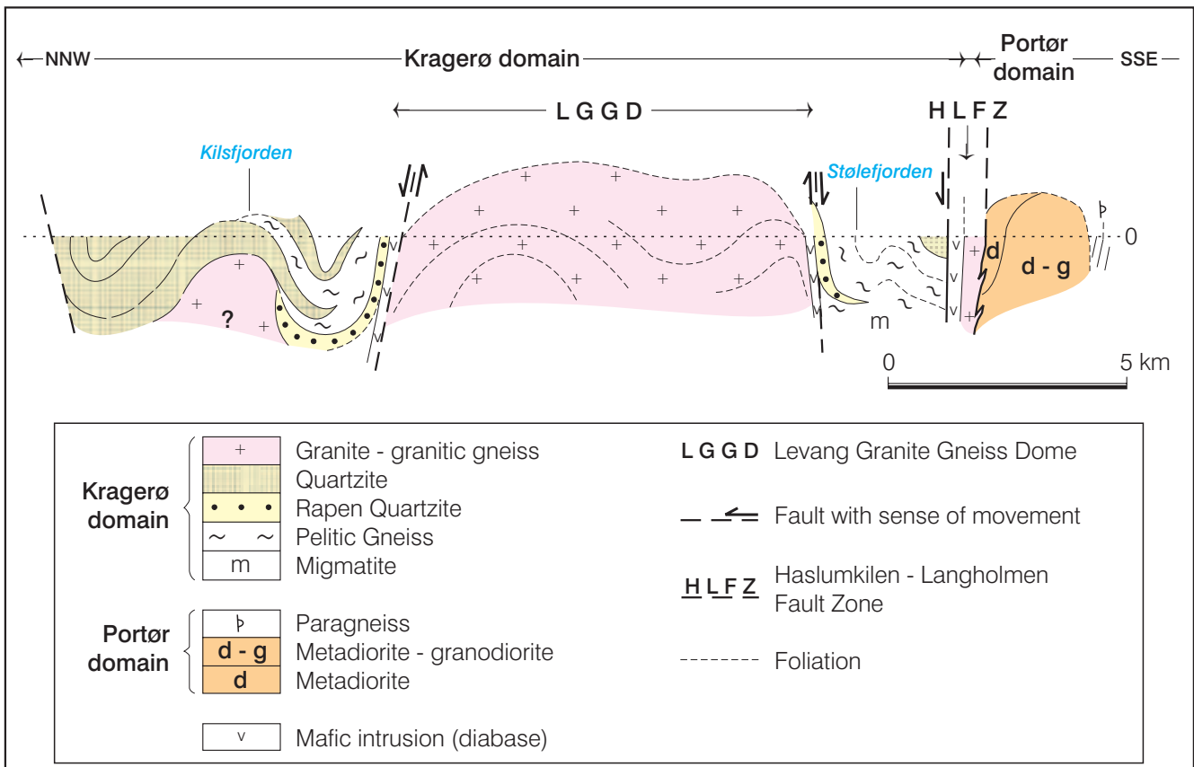
Fig 7. Cross-section (schematic) over the Levang Granite Gneiss Dome and associated rocks of the Kragerø and Portør domains showing some of the main structural features. Note the folding of the foliation planes in the granite gneiss and steeply inclined marginal faults. The latter may be an indication of some upward, diapiric rise of the granite gneiss body.
