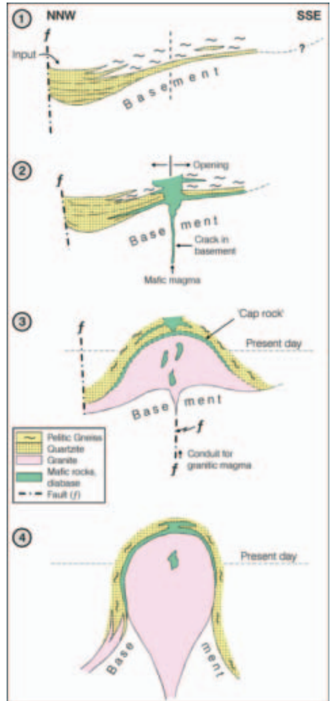
Fig. 8. Schematic drawings to demonstrate the early evolution of the Levang Granite Gneiss Dome. 1) depositional phase, 2) intrusion of mafic magma, 3) main granite intrusion. The configuration of the granite at depth is uncertain, 4) a more pear-shaped form, narrowing downwards, is also possible.
