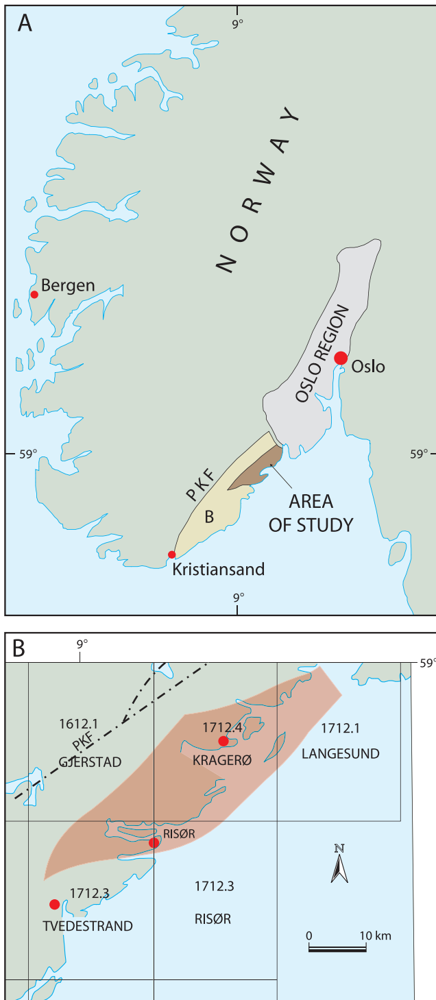
Fig 1. Maps showing location of the area of study in southern Norway; (A) its location in the Bamble Sector. B – Bamble Sector, PKF - Porsgrunn-Kristiansand Fault Zone; (B) relation to the 1:50,000 bedrock map-sheets.
