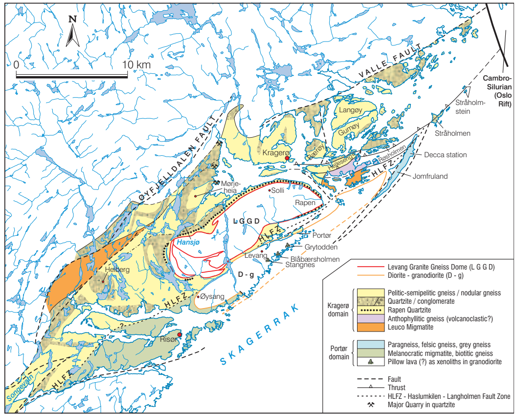
Fig 4. Distribution of the main metasedimentary rock formations in the Kragerø and Portør domains. The major mafic intrusions are omitted.
