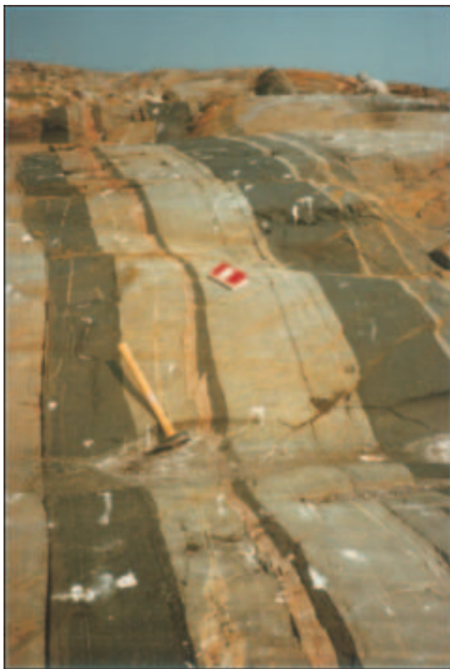
Fig 11. Paragneisses (?metasediments) of uncertain origin, invaded by diabasic dykes (dark in photo). The parallelism achieved is broken by minor transverse faults. Coastal exposures on the SE shore of Jomfruland, close to the Decca station. (Portør domain).
