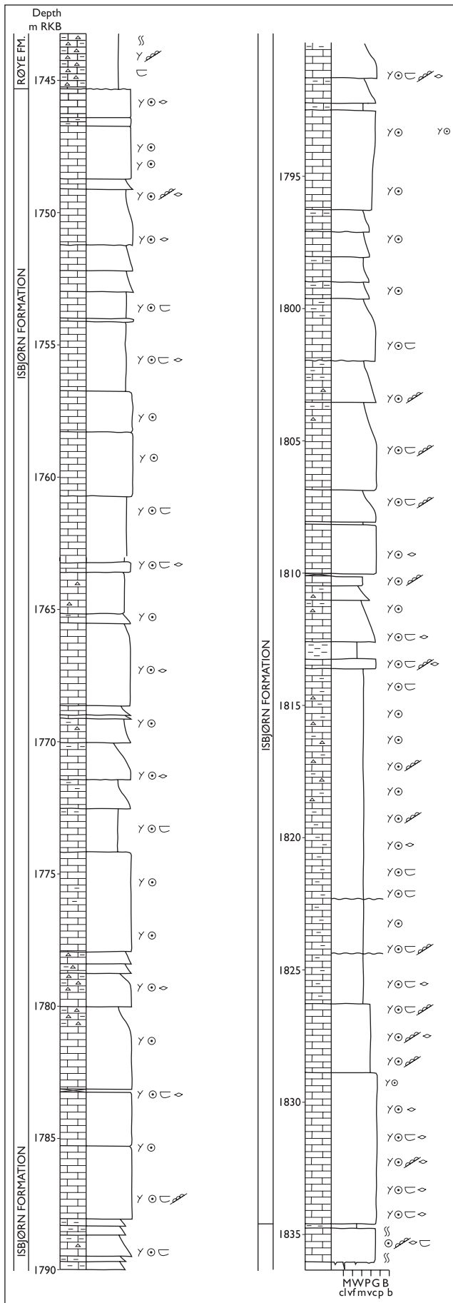
Fig. 22. Sedimentological log of the Isbjørn Formation in the type section in well 7128/6-1, Finnmark Platform. The succession is composed of well-bedded, bryozoan-crinoid-brachiopod wackestones and packstones typical of Late Palaeozoic, cool-water, carbonate shelves. For explanation of symbols, see Fig. 3.
