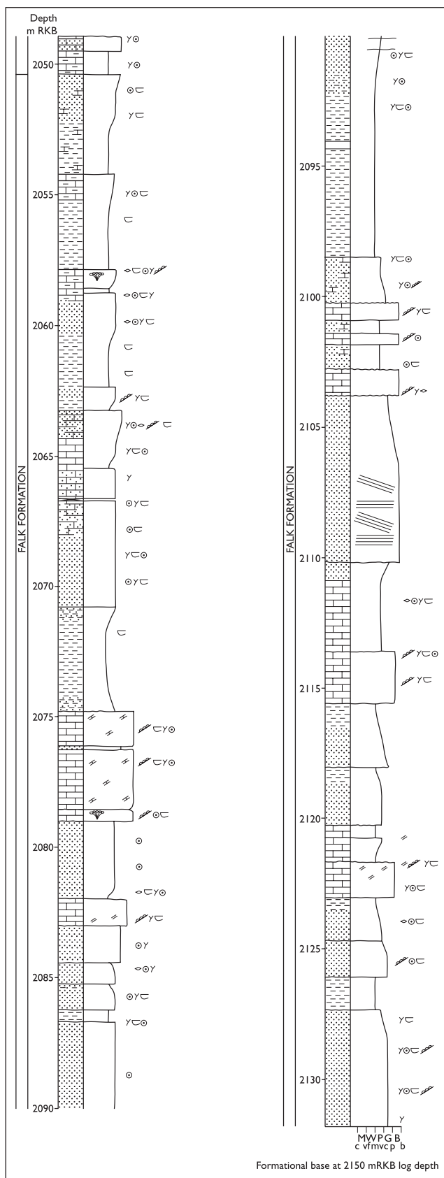
Fig. 15. Sedimentological log of the Falk Formation in reference well 7128/6-1 illustrating the characteristic interbedding of carbonates and marine siliciclastics. The stratigraphic position of the cored interval is shown in Fig. 11. For explanation of symbols, see Fig. 3.
