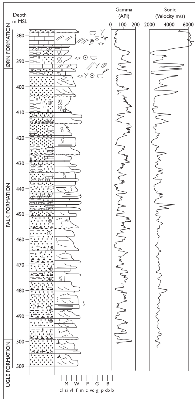
Fig. 13. Sedimentological log of the Ugle and Falk formations in reference core 7029/03-U-02. The stratigraphic position of the cored interval is shown in Fig. 11. For explanation of symbols, see Fig. 3.
