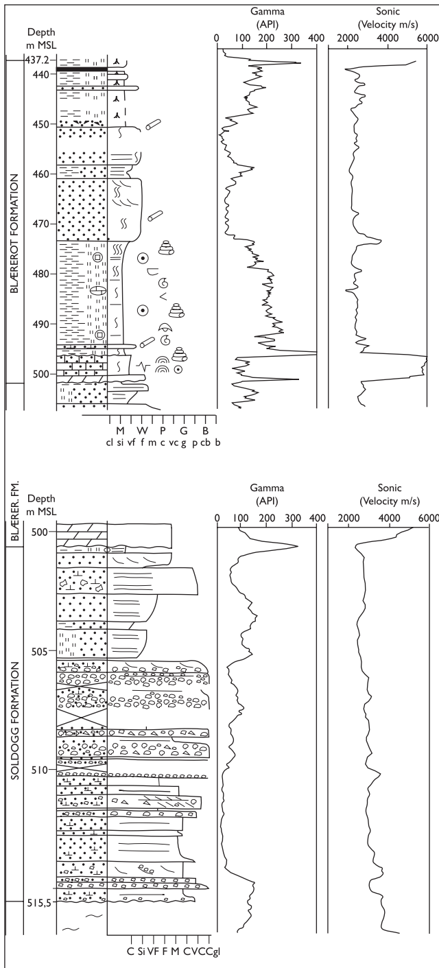
Fig. 9. Sedimentological log of the Soldogg and Blærerot Formations in core 7029/03-U-01 illustrating the basal marine limestone and mudstone succession of the Blærerot Formation. The stratigraphic position of the cored interval is shown in Fig. 6. For explanation of symbols, see Fig. 3.
