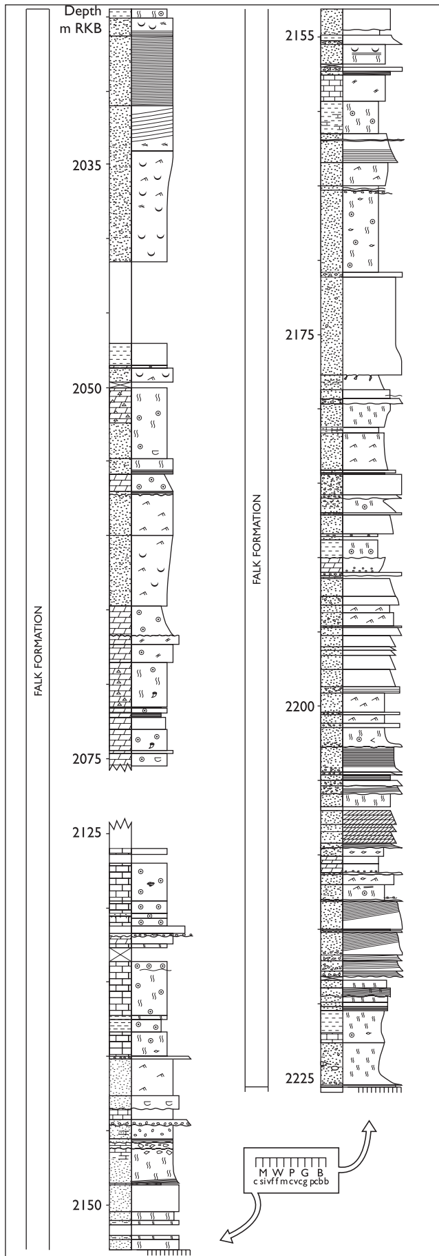
Fig. 14. Sedimentological log of the cored part of the Falk Formation in its type section in well 7120/2-1, Loppa High. Reproduced from Stemmerik et al. (1998) with permission from Norsk Petroleumsforening. The stratigraphic position of the cored interval is shown in Fig. 11. For explanation of symbols, see Fig. 3.
