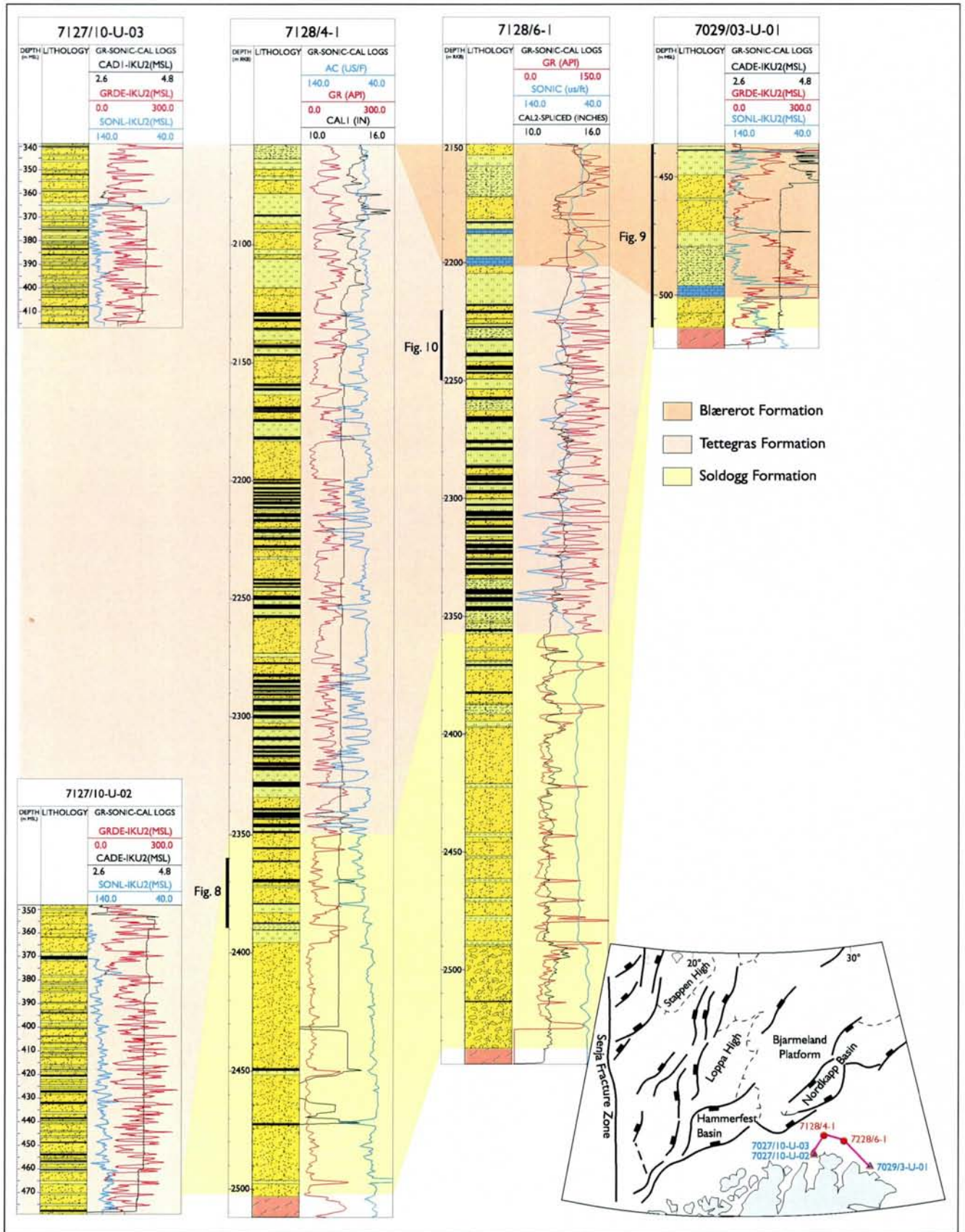
Fig. 6. Correlation of the Billefjorden Group on the Finnmark Platform. The position of cored sections illustrated by sedimentological logs in Figs 8–10 is indicated by black bars. For explanation of symbols, see Fig. 3.
