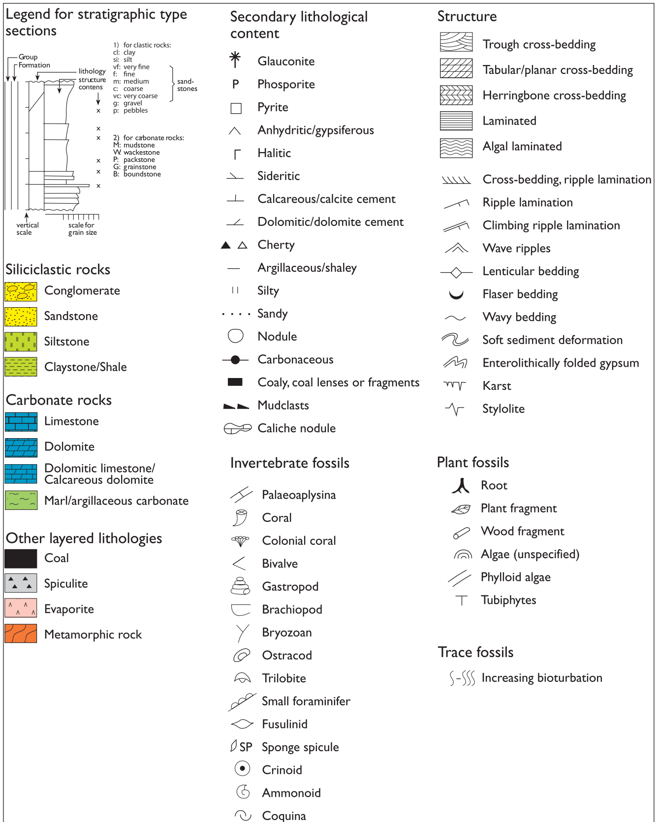
Fig. 3. Legend to well logs and core descriptions.
