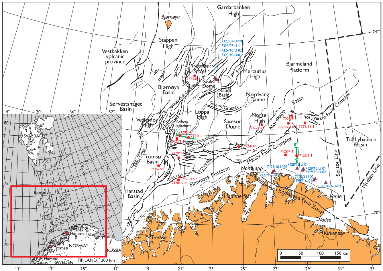
Fig. 1. Map of the southern Norwegian Barents Sea showing main structural elements and location of wells and shallow cores penetrating the Upper Palaeozoic succession. Position of seismic lines in Fig. 5 is shown.
