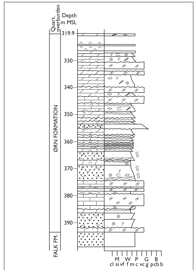
Fig. 18. Sedimentological log of the Ørn Formation in reference core 7029/03-U-02. The stratigraphic position of the cored interval is shown in Fig. 11. For explanation of symbols, see Fig. 3.
