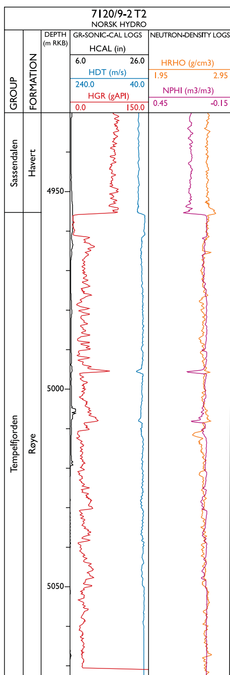
Fig. 24. Well logs of the upper part of the Tempelfjorden Group in 7120/9-2, Hammerfest Basin, showing the boundary to the Triassic Havert Formation. For explanation of symbols, see Fig. 3.
