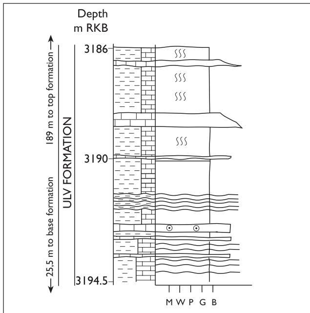
Fig. 21. Sedimentological log of the cored interval of the Ulv Formation in reference well 7120/1-1, Loppa High. For explanation of symbols, see Fig. 3.
