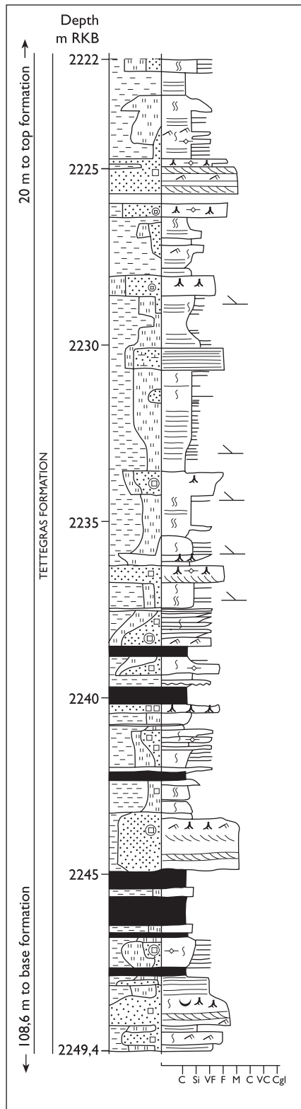
Fig. 10. Sedimentological log of the upper Tettegras Formation in well 7128/6-1 showing fluvial fining-upwards cycles, some of which are capped by coal. The stratigraphic position of the cored interval is shown in Fig. 6. For explanation of symbols, see Fig. 3.
