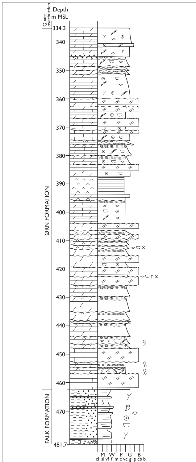
Fig. 17. Sedimentological log of the Falk and Ørn formations in reference core 7030/03-U-01 illustrating the facies variations of the completely dolomitised warm-water carbonate succession. The stratigraphic position of the cored interval is shown in Fig. 11. For explanation of symbols, see Fig. 3.
