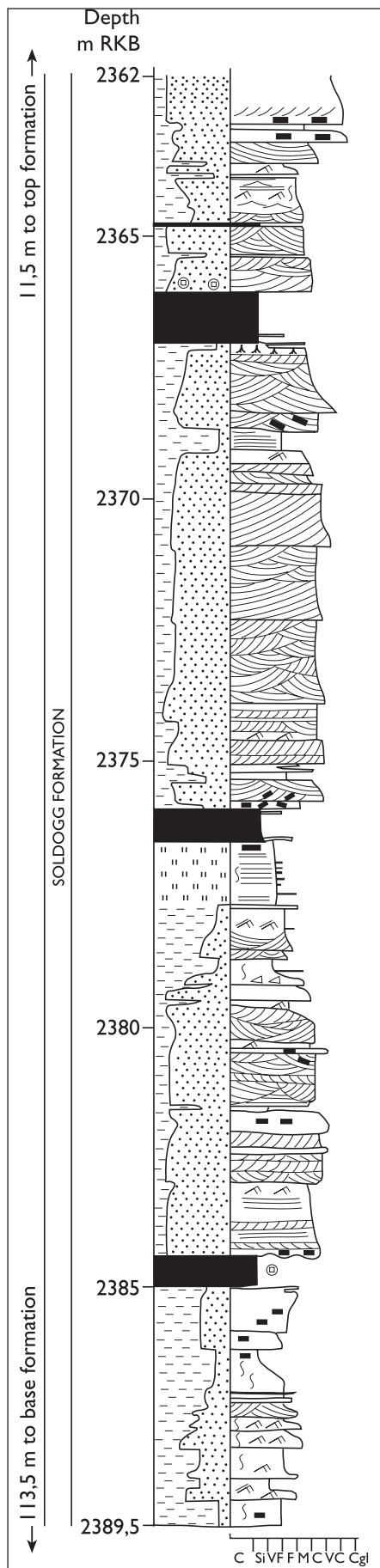
Fig. 8. Sedimentological log of the upper Soldogg Formation, well 7128/4-1 showing coal-capped, fluvial, fining-upward cycles. The stratigraphic position of the cored interval is shown in Fig. 6. For explanation of symbols, see Fig. 3.
