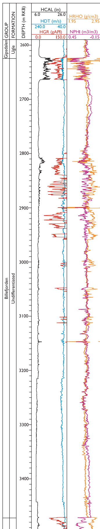
Fig. 7. Well logs of the succession assigned to the Billefjorden Group in well 7120/2-1 from the Loppa High. For position, see Fig. 1.
