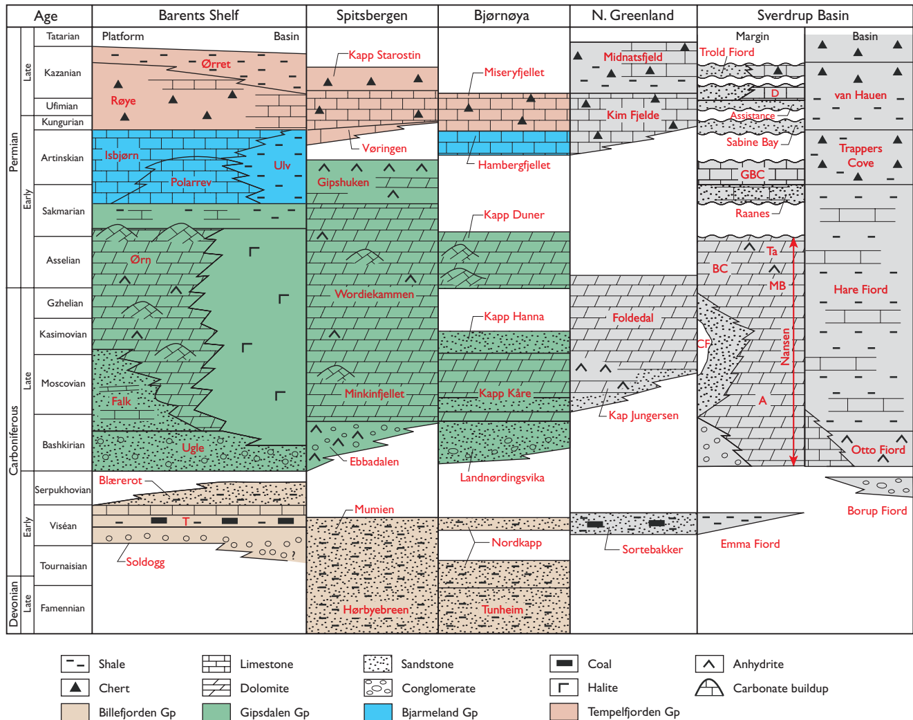
Fig. 25. Correlation of Upper Palaeozoic lithostratigraphic units between Norwegian onshore and offshore areas, North Greenland and Arctic Canada. Based on Dallmann et al. (1999), Stemmerik (2000), Dalhoff et al. (2000) and Beauchamp et al. (2001). A: Antoniette, D: Degerbøls, T: Tettegras, BC: Belcher Canyon, CF: Canyon Fiord, MB: Mount Bayley, Ta: Tanquary, GBC: Great Bear Cape.
