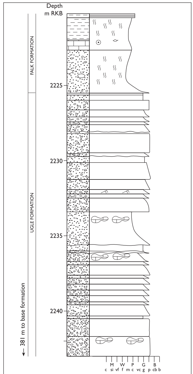
Fig. 12. Sedimentological log of the uppermost Ugle Formation in its type section in well 7120/2-1, Loppa High, illustrating the shift from caliche-capped alluvial conglomerates to marine sandstones and limestones. The stratigraphic position of the cored interval is shown in Fig. 11. For explanation of symbols, see Fig. 3.
