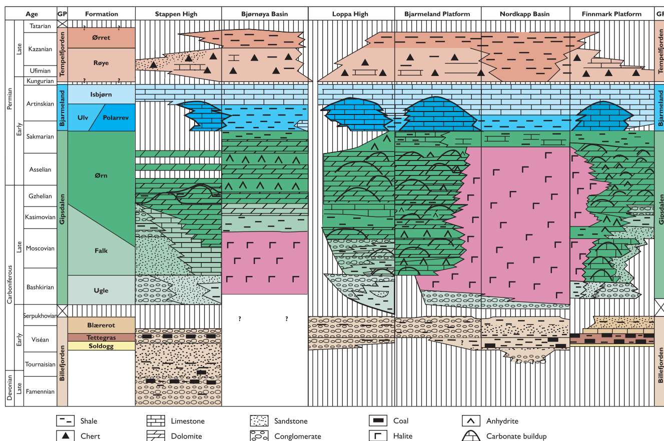
Fig. 4. Correlation of the Upper Palaeozoic lithostratigraphic units in the offshore areas of the southern Norwegian Barents Sea. The geographical distribution of lithostratigraphic units is based on a combination of well and seismic data. The background for age assignments are discussed in the text.
