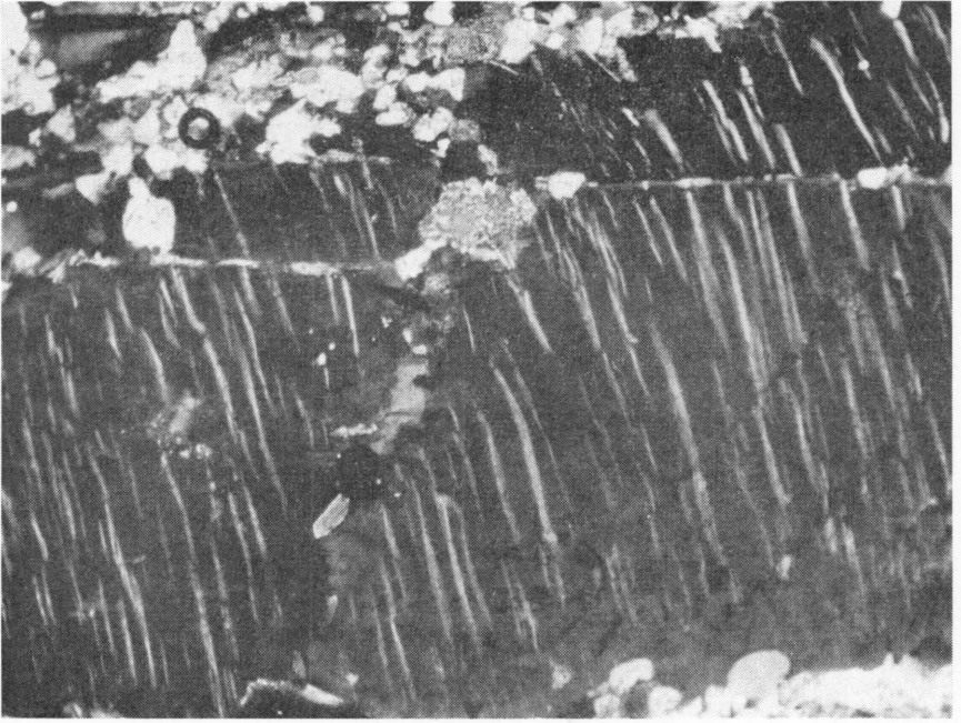
Photo No. 13. Deformed K-felspar in sheared, foliated granite (.35, crossed polars).
