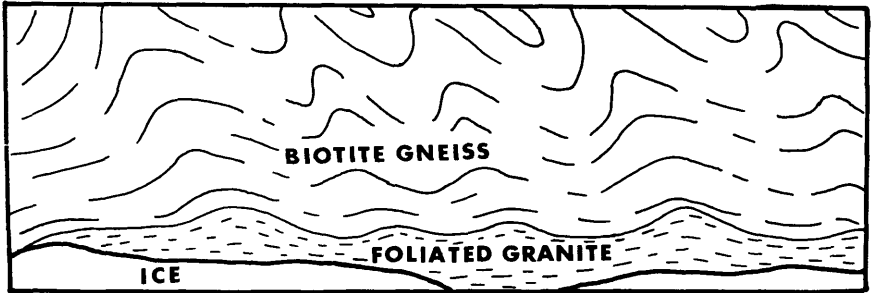
Fig. 38. The relationship between fold-styles, lithology and depth in the Høybreen side-wall section. Length of section — 300 metres.
