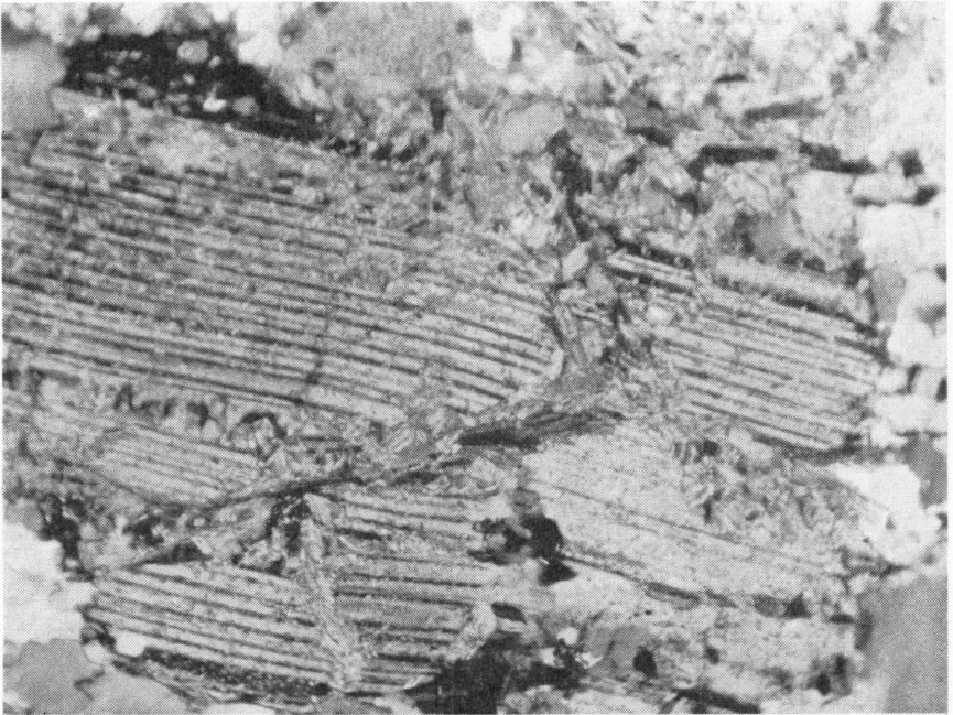
Photo No. 14. Plagioclase with muscovite on planes of dislocation in sheared, foliated granite. (x35, crossed polars).
