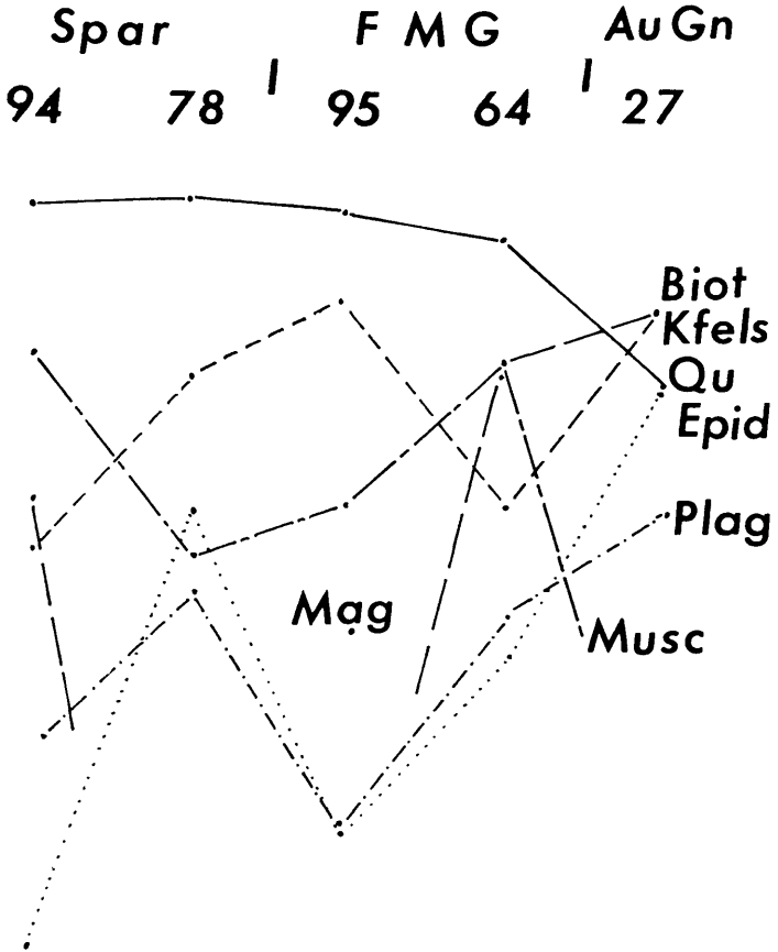
Fig. 34. Mineralogical traverse across the basement contact (Sparagmite / flaggy, muscovite gneiss / augen gneiss.)
