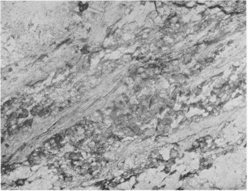
Photo No. 15. Muscovite bearing planes disrupting K-felspar in schistose, muscovite gneiss, (x35 plane polarised light).
