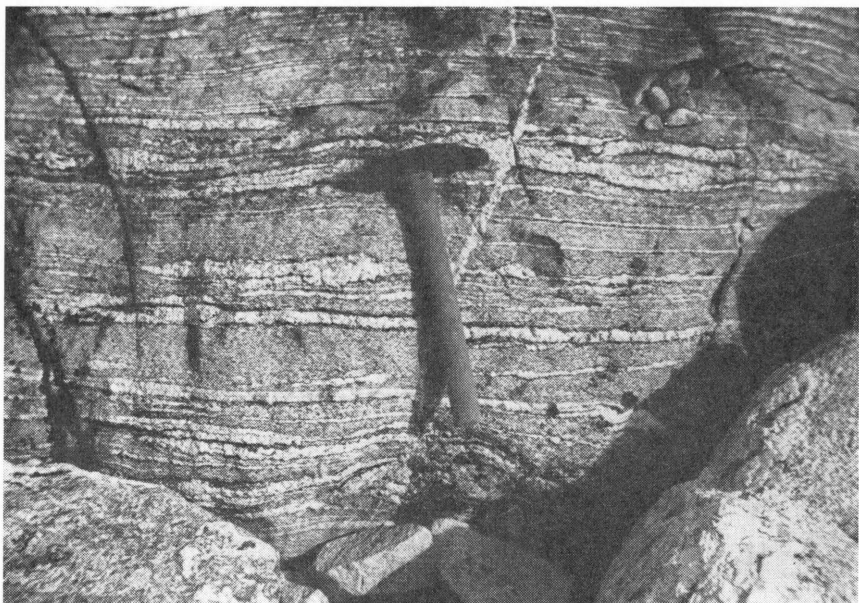
Photo No. 1. Typical, banded, biotite gneiss.
