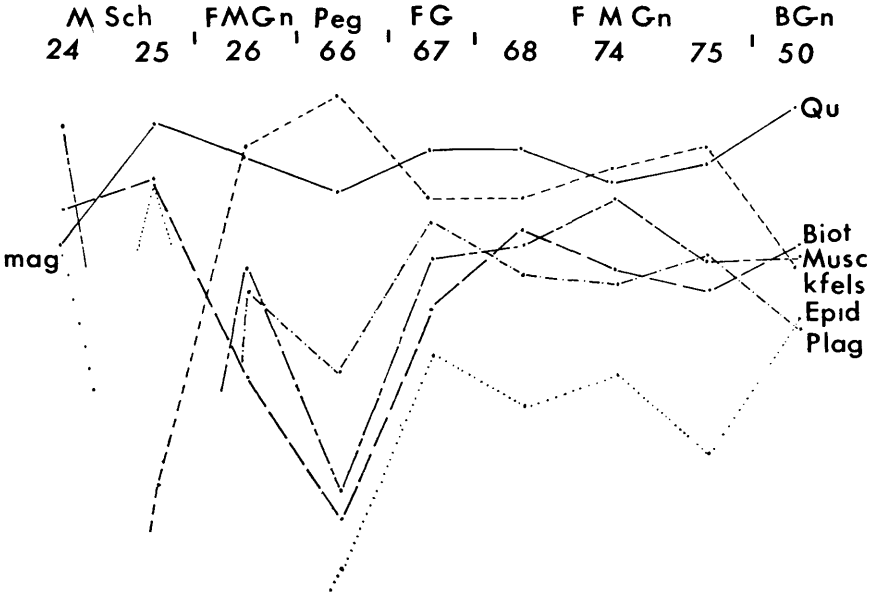
Fig. 32. Mineralogical traverse across the basement contact (mica-schist/flaggy, muscovite gneiss) and various other lithological boundaries (pegmatite, foliated granite and biotite gneiss with flaggy, muscovite gneiss).
