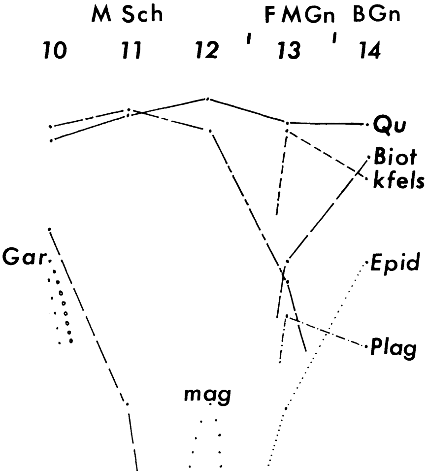
Fig. 33. Mineralogical traverse across the basement contact.
