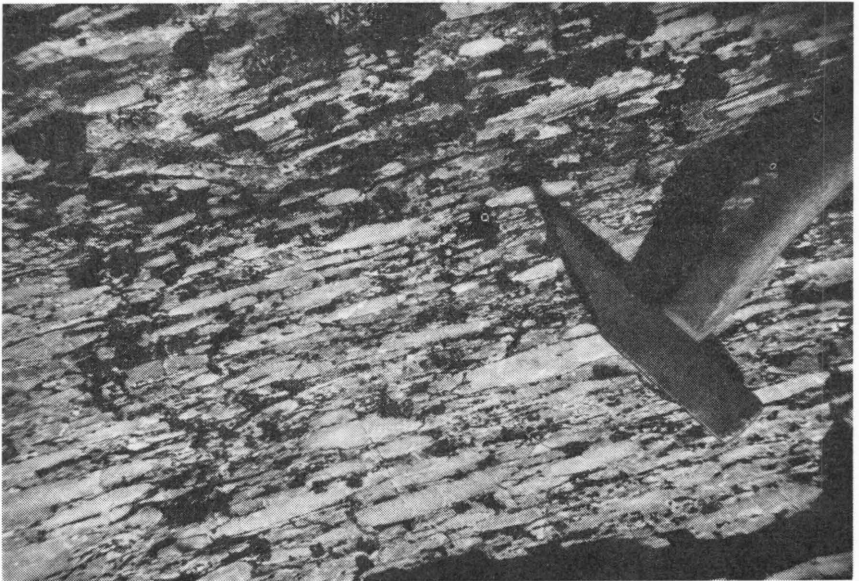
Photo No. 19. Deformed conglomed conglomerate (?) from Hesthøe (g.r. 572498).
