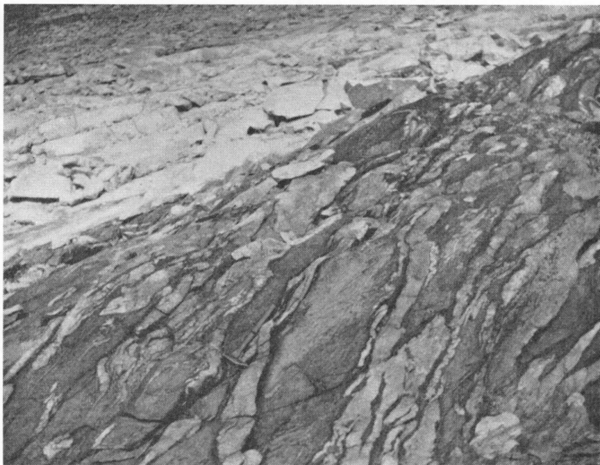
Photo No. 8. Granite veins in biotite gneiss xenolith, (Briedalen, g.r. 456431).
