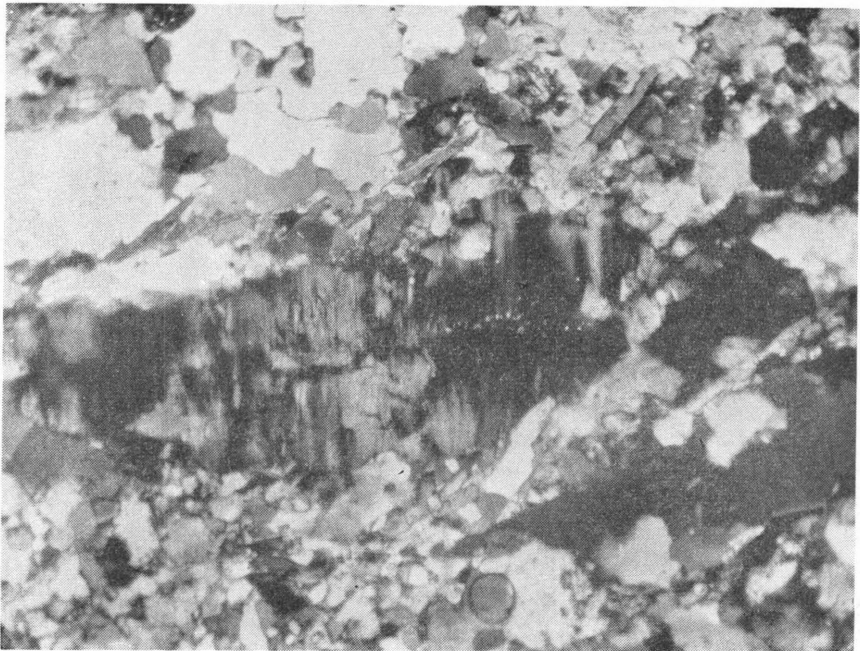
Photo No. 12. Undulose extinction in K-felspar in sheared, foliated granite (x35, crossed polars).
