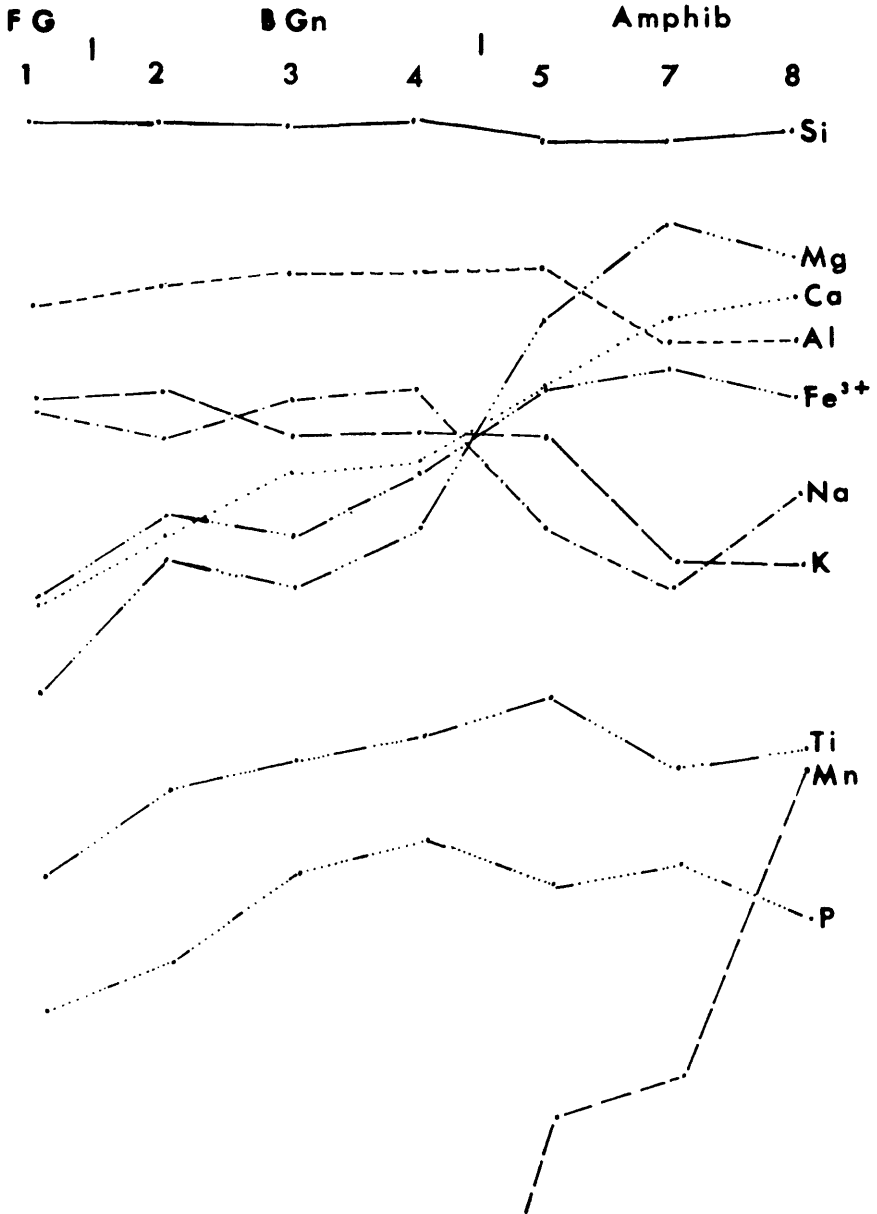
Fig. 21. Chemical traverse across biotite gneiss/ amphibolite contact.
