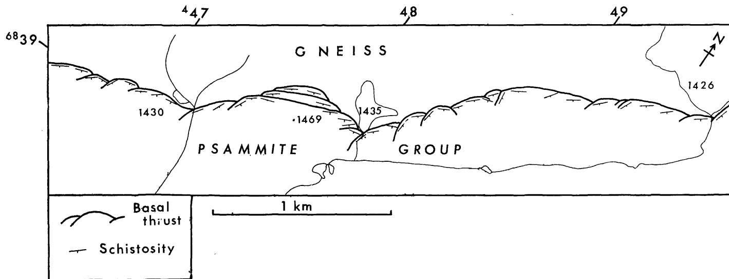
Fig. 41. A detailed map of a portion of the Basal thrust outcrop.
