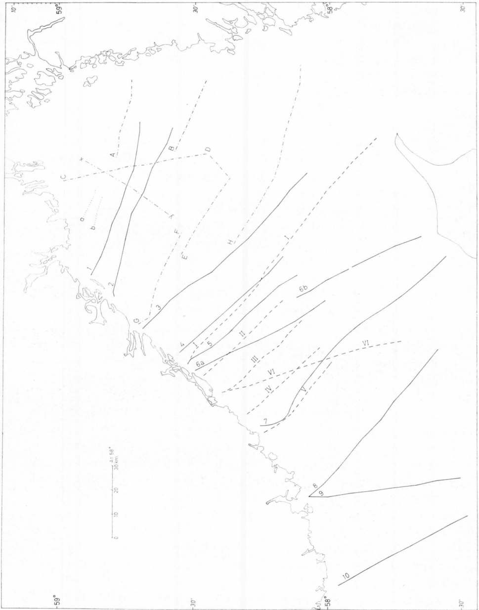
Fig. 1. Positions of profiles seen in fig. 2 (full drawn lines), in fig. 3-4 (--- 1955-56, --- 1960), and fig. 5 (. . . and -.-.). Cf. also main map, pl. 1.
