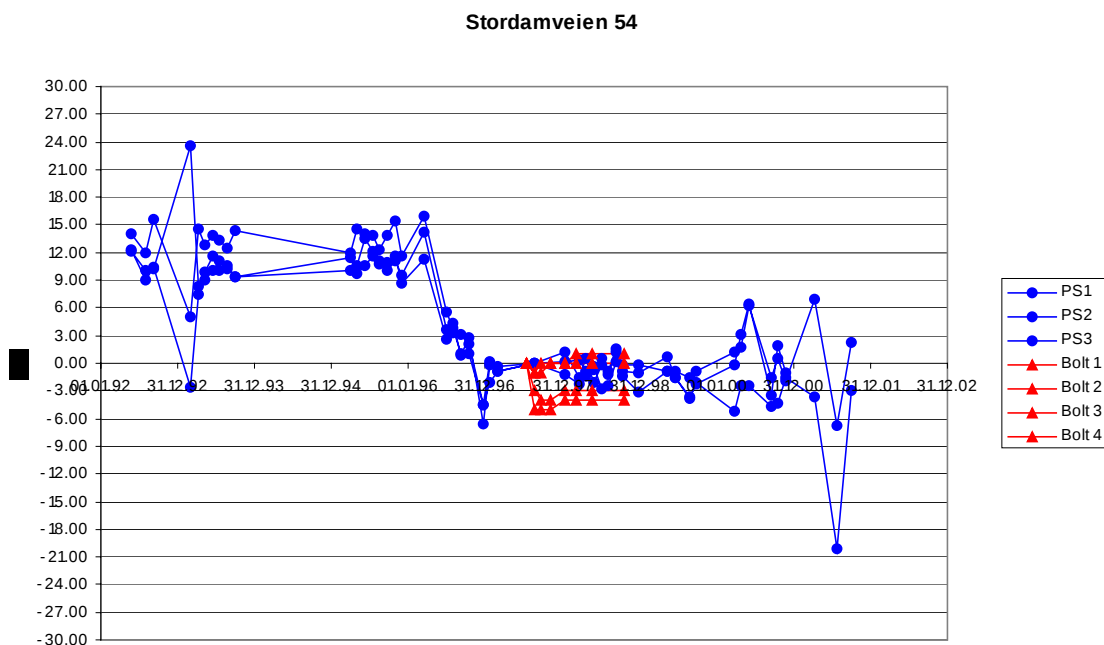
Figure 25. Subsidence measured in Stordamveien 54 by levelling compared with three PS from the same building. Although the signal-to-noise ratio is low, PS measurements reveal subsidence not detected by levelling, which began only afterwards. Blue dots are from PS. Red triangles are from bolts on the corners of the house.
