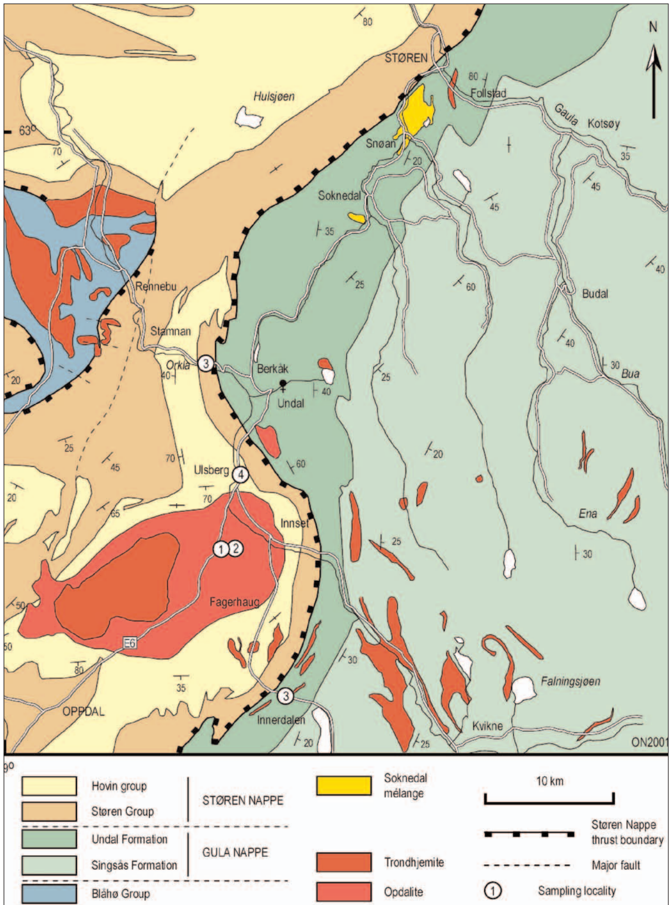
Fig. 2. Geological map of the Ulsberg-Kvikne- Soknedal district showing the locations of the samples (1-5) investigated in this geochronological/geochemical study.
