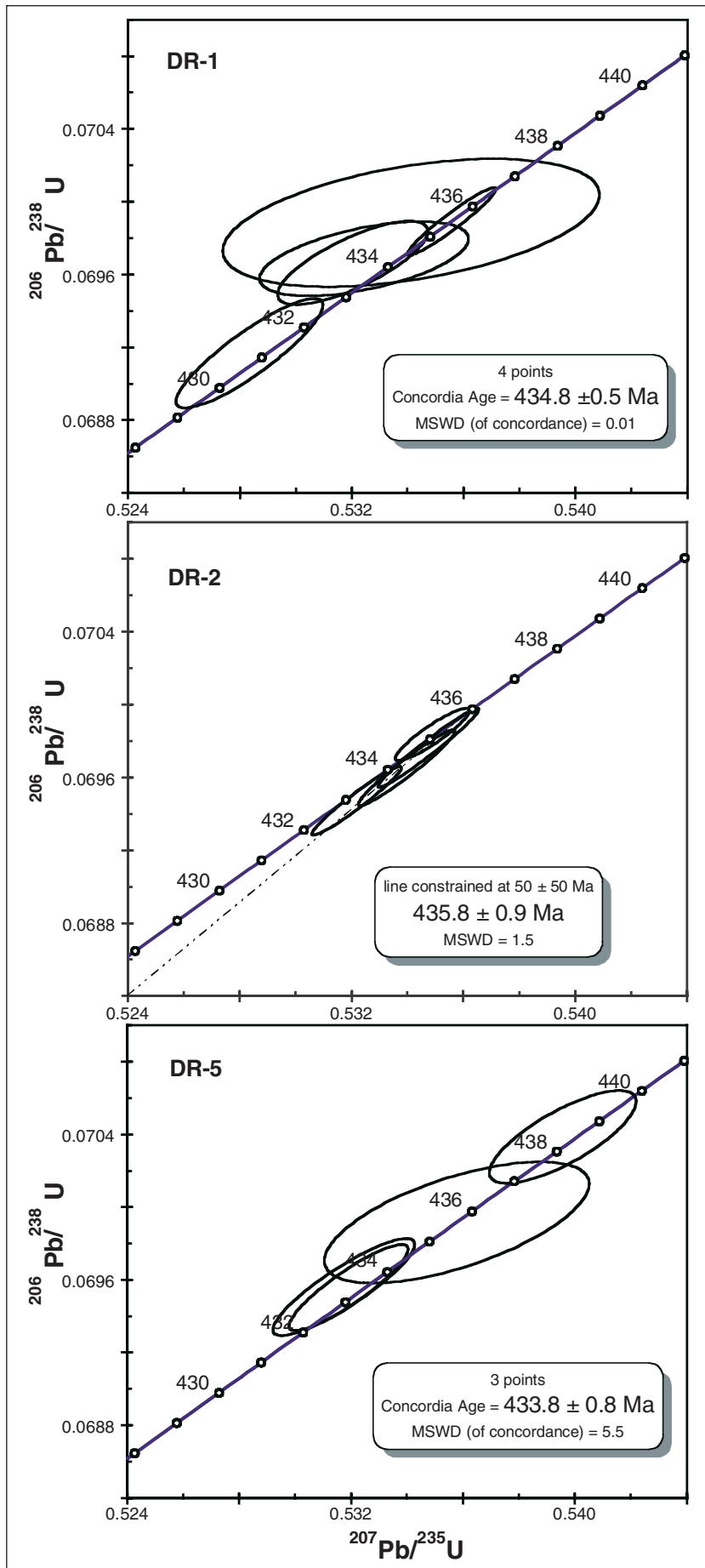
Fig. 7. Concordia diagrams for the zircons analysed from samples DR1, DR2 and DR5. See main text for explanation.
