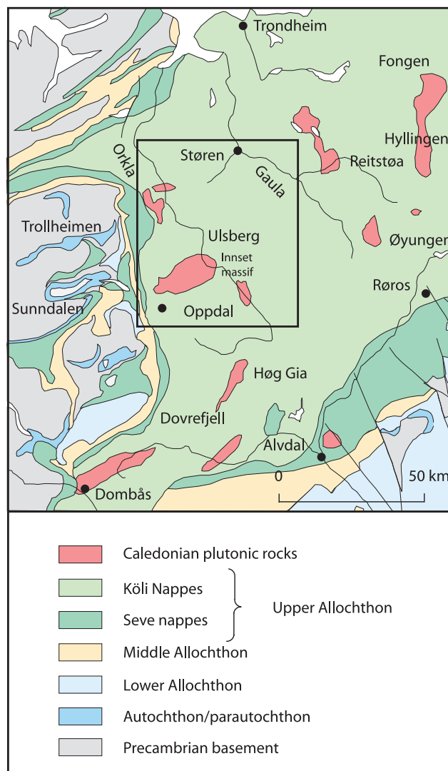
Fig. 1. Simplified tectonostratigraphy of the southwestern part of the Trondheim Region, showing the location of the area (box) depicted in Figure 2. Some of the principal trondhjemite or gabbro-diorite-trondhjemite massifs are also indicated.
