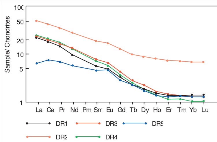
Fig. 6. Chondrite-normalised REE plots of the trondhjemites and biotite norite from the Berkåk-Innset-Innerdal area. Element normalisation values from Taylor & McClellan (1985).
