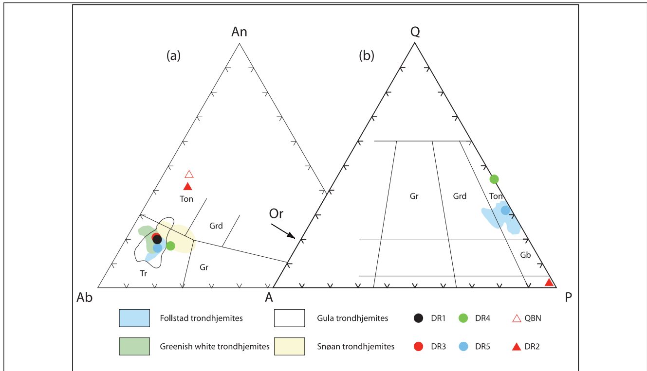
Fig. 4. (a) Normative (An-Ab-Or) and (b) modal (Q-A-P) diagrams of trondjemites and associated rocks from the west-central Trondheim Region. The An-Ab-Or diagram is from O'Connors (1965). Gr - granite; Grd - granodiorite; Ton - tonalite; Qgb - quartz gabbro; Gb - gabbro/diorite. The fields of 'Follstad trondjemites' and 'Greenish-white trondjemites' are from Pannemans & Roberts (2000) (normative) and Size (1979) (modal); and the 'Snøan trondjemites' from Roberts & Sundvoll (2000). The field for 'Gula trondjemites' (12 samples) encompasses analyses by Goldschmidt (1916) and O. Nilsen (unpublished data). QBN - One quartz-biotite norite sample from the Innset massif, taken from Goldschmidt (1916) (modal analysis not available).
