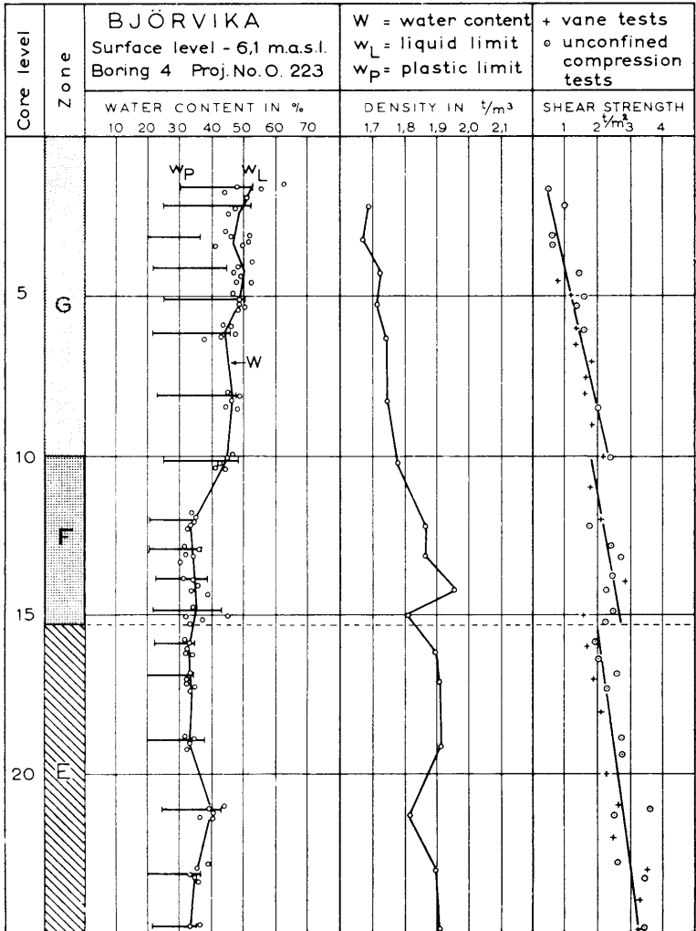
Fig. 5 Stratigraphy and geotechnical properties of clay sediments at the inner harbour of Oslo, as revealed by a 25 m deep boring at Bjørvika.
