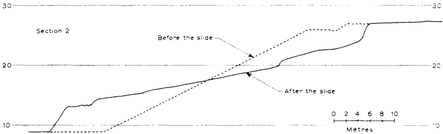
Fig. 19. Profile of the landslide at Lodalen, Oslo, section 2 in fig. 18.
