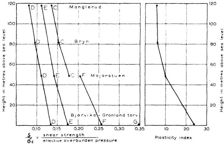
Fig. 8. a) Variation of the ratio shear strength to effective overburden pressure, s/\sigma_c , for the different stratigraphic zones of 10 borings from Oslo, with the elevation at which the deposits are found. b) Variation of plasticity index for some clay deposits from Oslo (see table p. 26) with the elevation above sea level at which the deposits are found.
