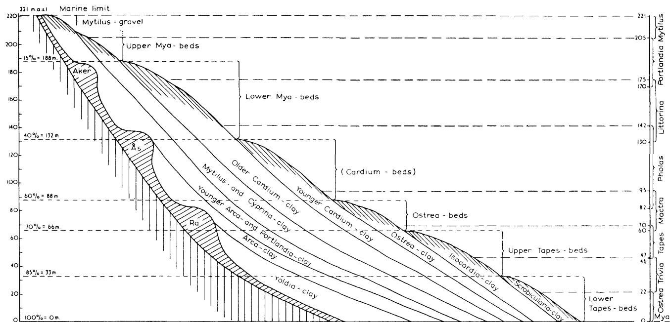
Fig. 3. Schematic illustration of the marine Late Pleistocene deposits of the Oslo region according to Brøgger's stratigraphy (slightly modified). To the right Øyen's shoreline stages. The heights above sea level refer to Oslo, they have also been indicated as percentages of the total elevation of the land. Morainic stages are also indicated. (Constructed in cooperation with O. Holtedahl and H. Rosendahl.)
