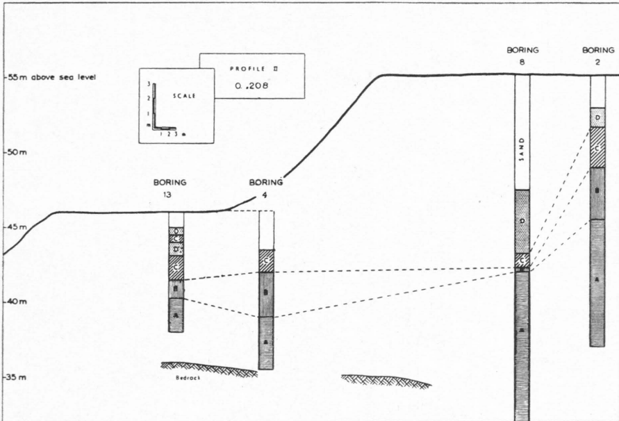
Fig. 13. Profile II, Høysskoleplatået (see fig. 12) with the borings projected into the same profile. The white parts of the cores have not been micropaleontologically investigated, they consist of coarse sand.
