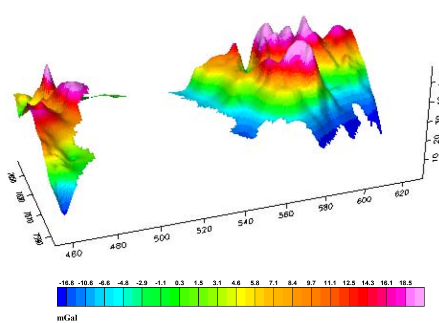
GRAVIMETRISK 3D RESIDUALKART GRAVITY 3D RESIDUAL MAP
