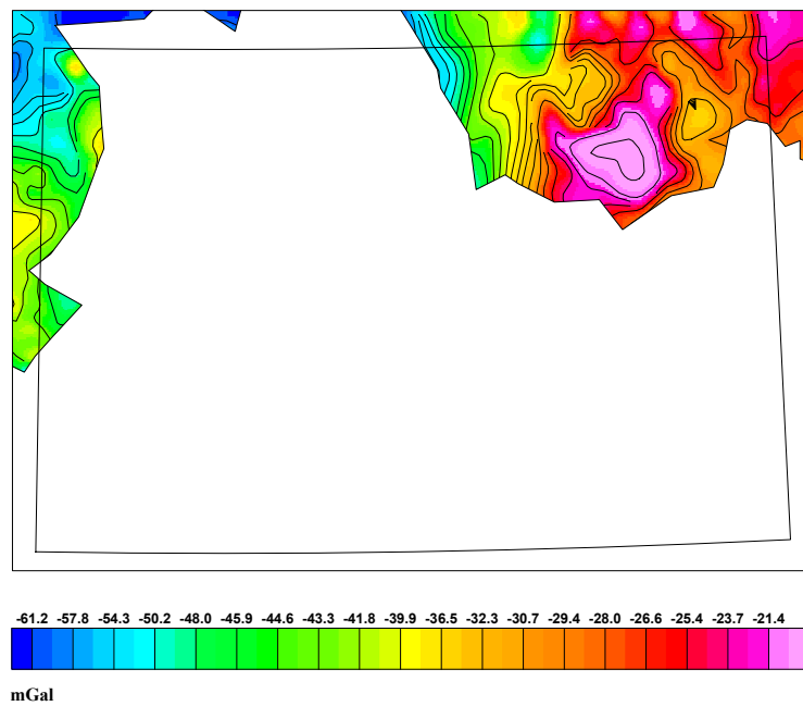
TYNGDEANOMALKART Terrengkorrigerte bougeranomalier GRAVITY ANOMALY MAP Terrain-corrected bouger anomalies
