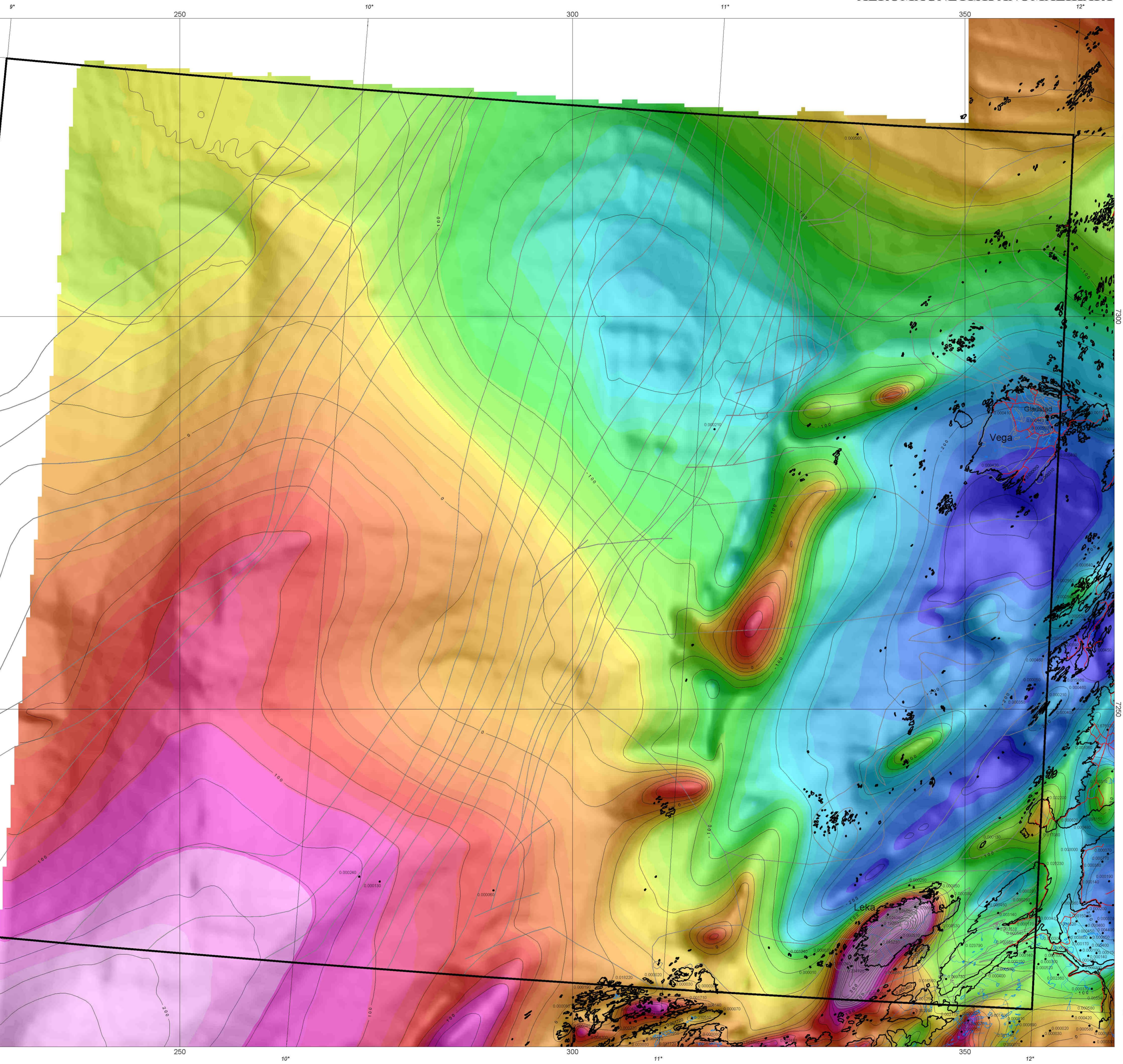
TYNGDEANOMALIKART Terrengkorrigerte bouguer-anomalier GRAVITY ANOMALY MAP Terrain-corrected bouguer anomalies
