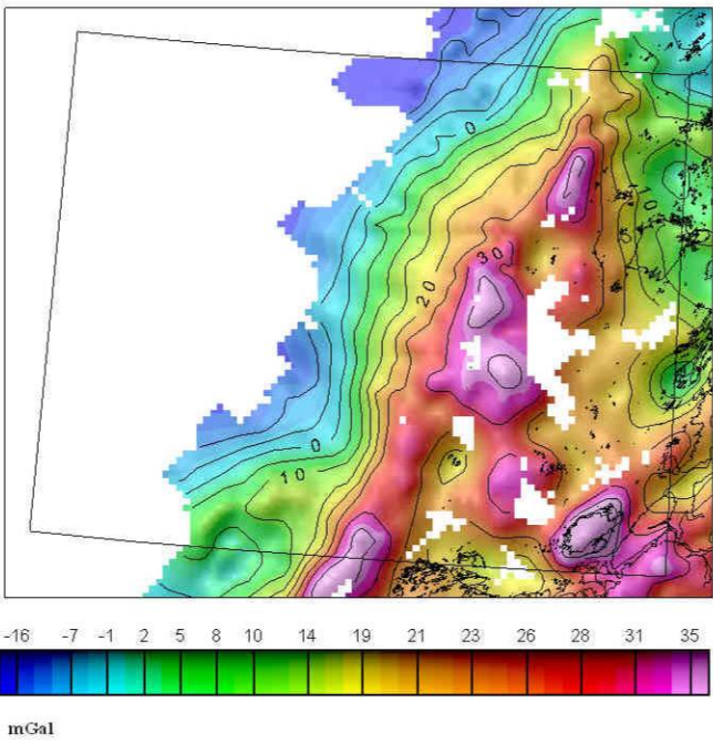
GRAVIMETRISK RESIDUALKART GRAVITY RESIDUAL MAP
