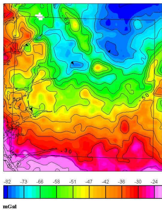
TYNGDEANOMALIKART Terrengkorrigerte bogseranomalier GRAVITY ANOMALY MAP Terrain-corrected bogser anomalies
