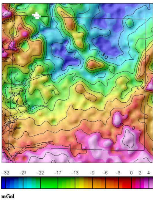
GRAVIMETRISK RESIDUALKART GRAVITY RESIDUAL MAP
