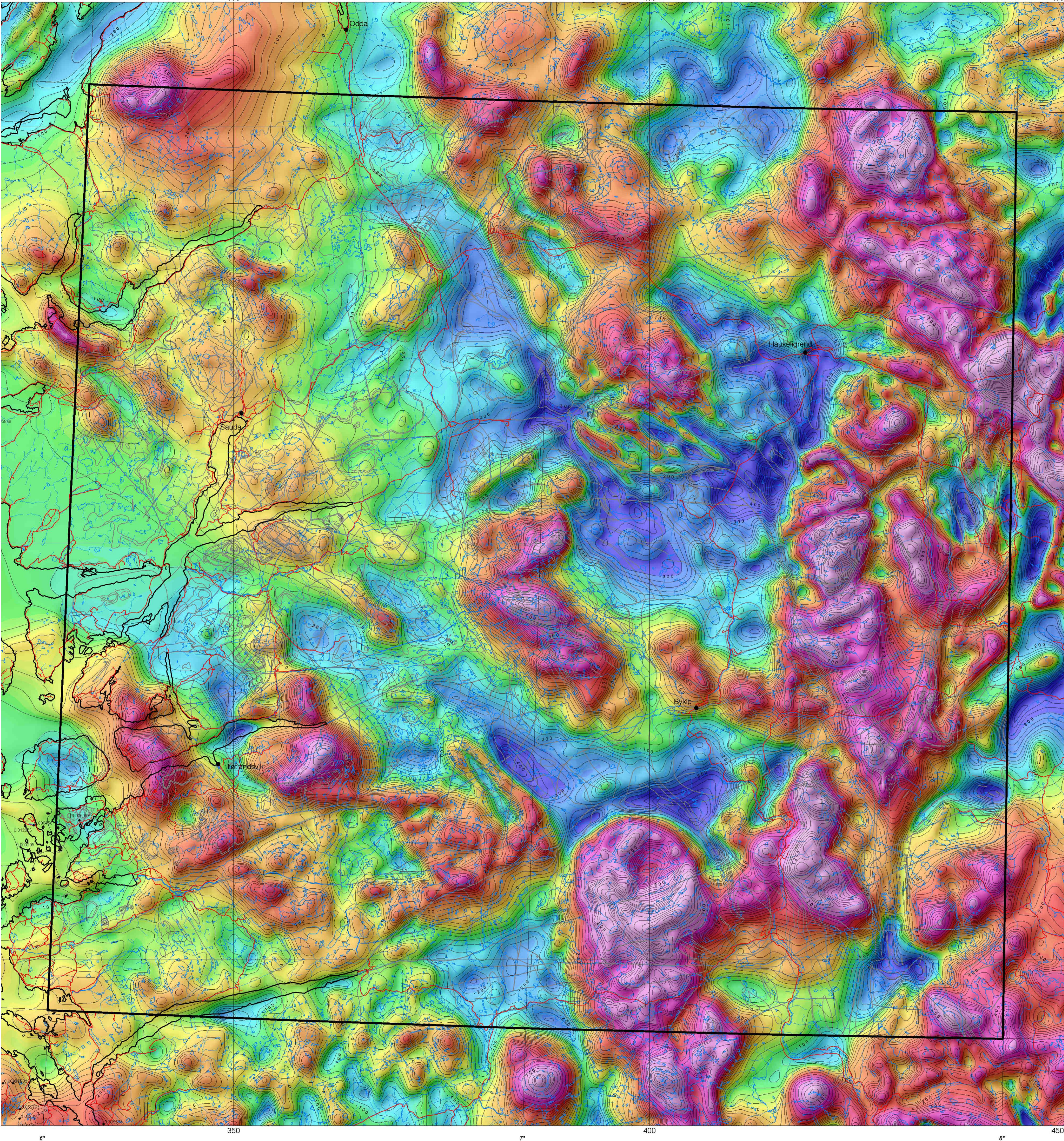
TYNGDEANOMALIKART Terrengkorrigerte bogseranomalier GRAVITY ANOMALY MAP Terrain-corrected bogser anomalies
