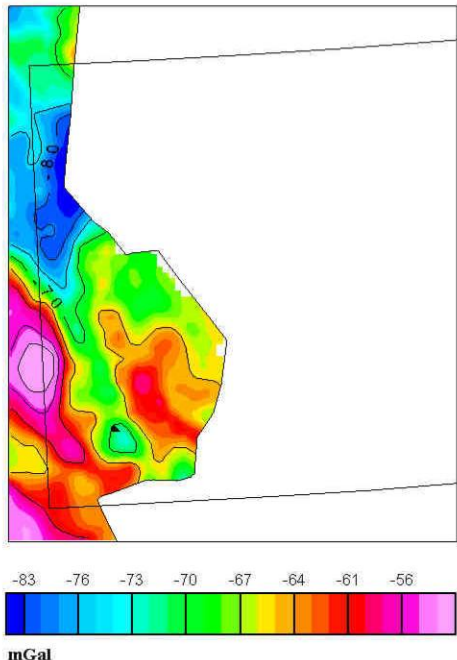
TUNGDIAEROMALIKART Terrenghøiregerte langper anomalies GRAVITY ANOMALY MAP Terrain-corrected langmuir anomalies
