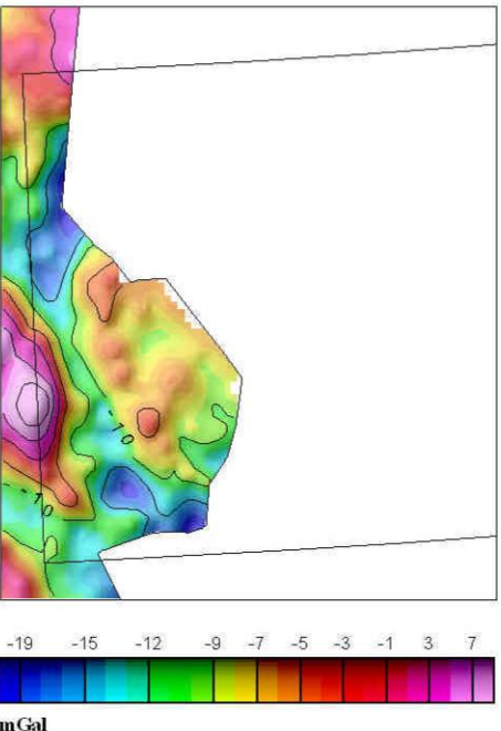
GRAVITETRISK RESIDUALKART GRAVITY RESIDUAL MAP
