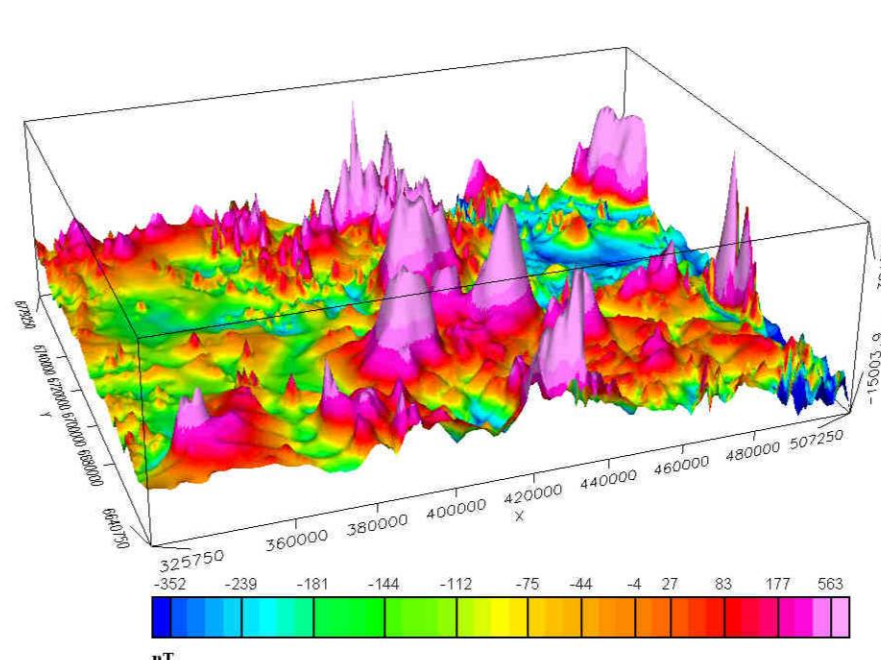
AEROMAGNETISK ID-ANOMALIKART Magnetfelt referert til DGRF 1965.0 AEROMAGNETIC ID-ANOMALY MAP Magnetic field referred to DGRF 1965.0
