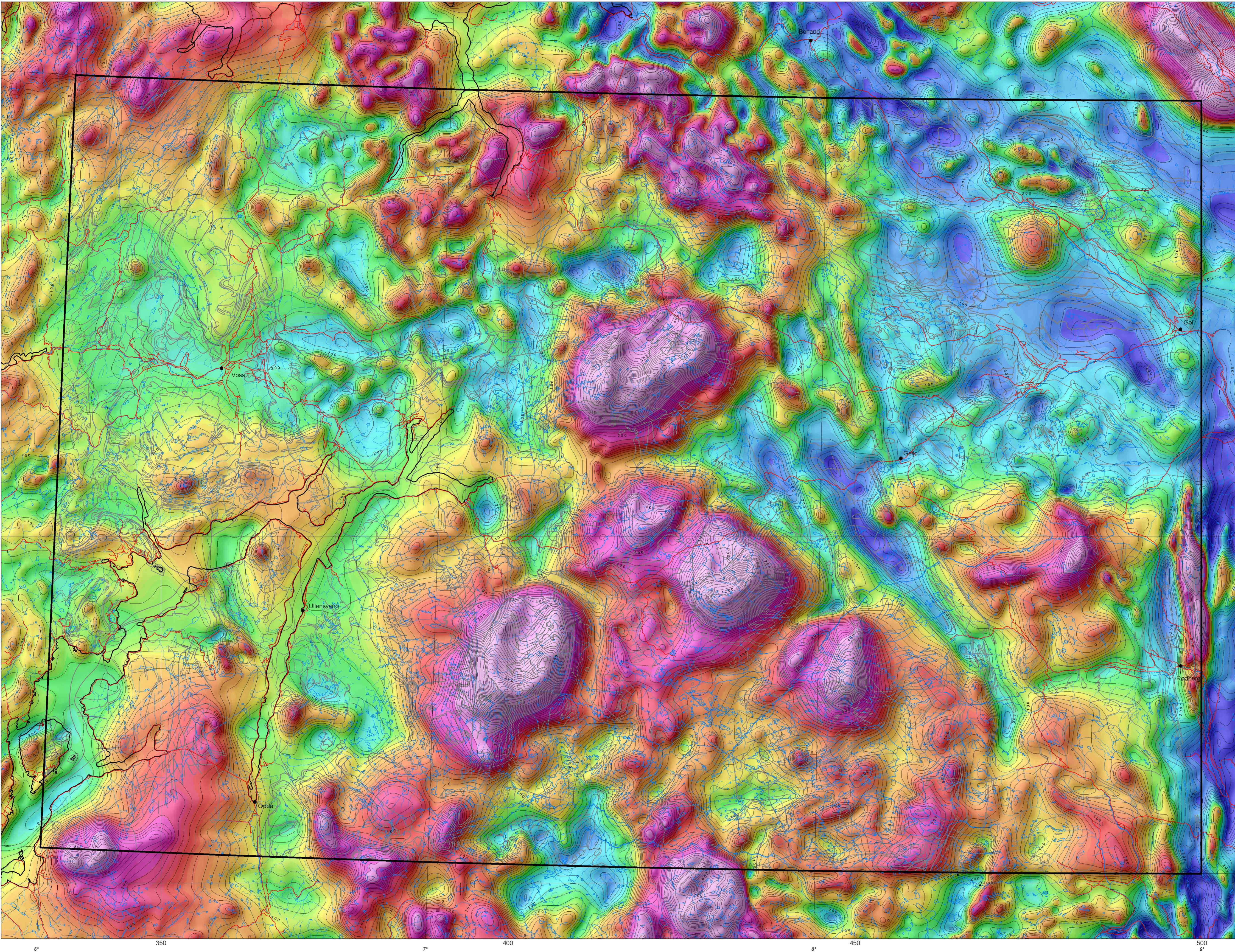
TYNGDEANOMALIKART Terrengkorrigerte magnetiske anomalier GRAVITY-ANOMALY MAP Terrain-corrected magnetic anomalies
