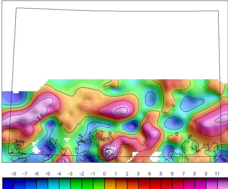
GRAVIMETRISK RESIDUALKART GRAVITY RESIDUAL MAP
