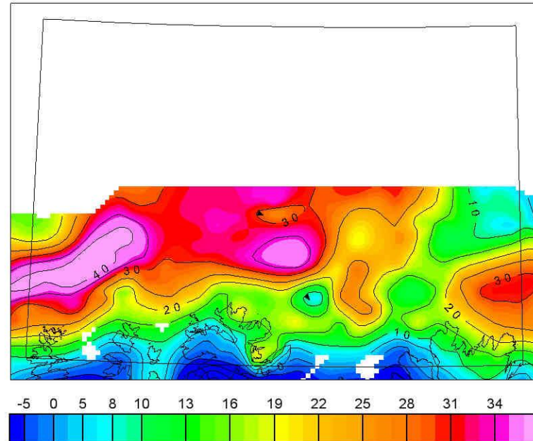
TYNGDEANOMALIKART Topographic gravity anomalies GRAVITY ANOMALY MAP Terrain-corrected bouguer anomalies
