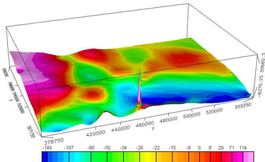
AEROMAGNETISK 3D ANOMALIKART Magnetic field referred to DGRF 1965.0 AEROMAGNETIC 3D ANOMALY MAP Magnetic field referred to DGRF 1965.0
