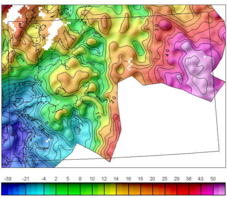
GRAVITETRESKE RESIDUALKART GRAVITY RESIDUAL MAP
