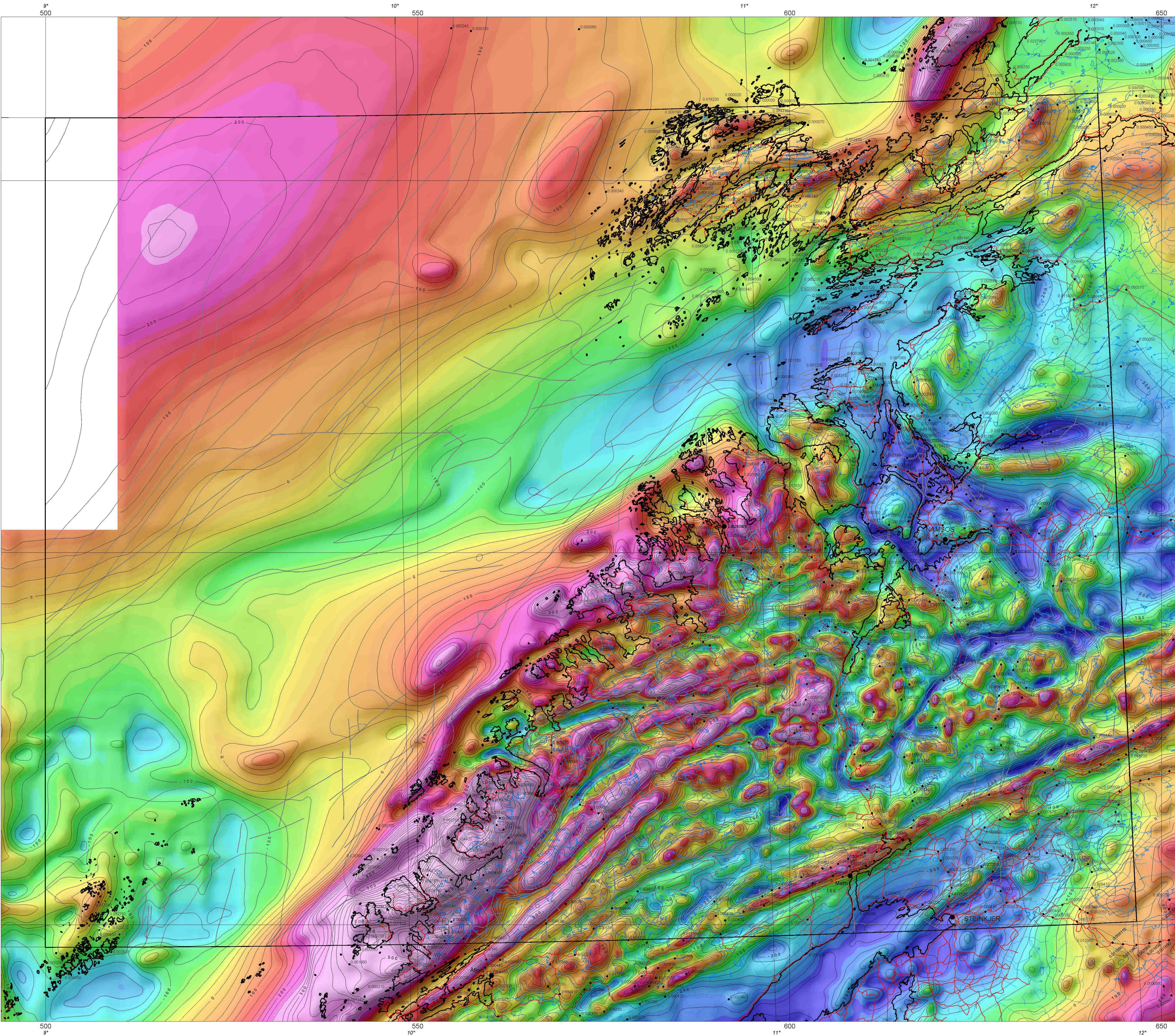
TYNGDEANOMALIKART Terrengkorrigerte topografiske anomalier GRAVITY ANOMALY MAP Terrain-corrected topographic anomalies
