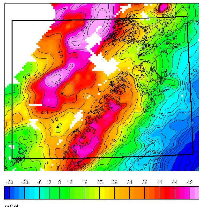
TYNGDEANOMALIKART Terrengkorrigerte topografiske anomalier GRAVITY ANOMALY MAP Terrain-corrected topographic anomalies
