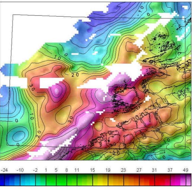
GRAVIMETRISKE RESIDUALKART Magnetfeltet referert til DGRF 1965.0 GRAVITY RESIDUAL MAP Magnetic field referred to DGRF 1965.0
