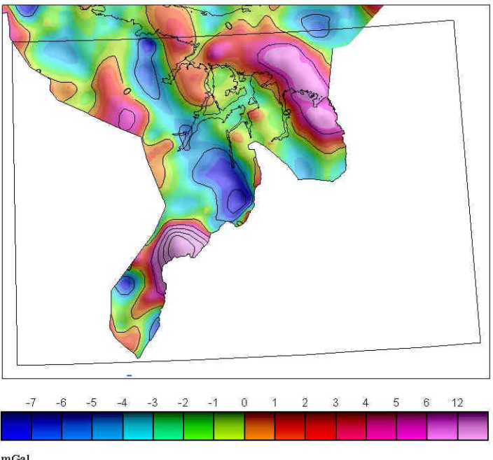
GRAVITRISK RESIDUALKART GRAVITY RESIDUAL MAP
