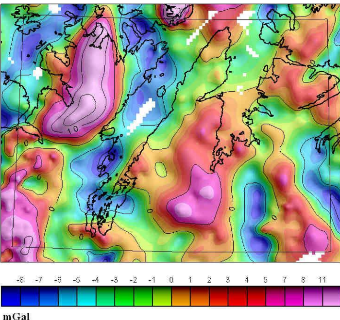
GRAVITETRISK RESIDUALKART Gravity residual map
