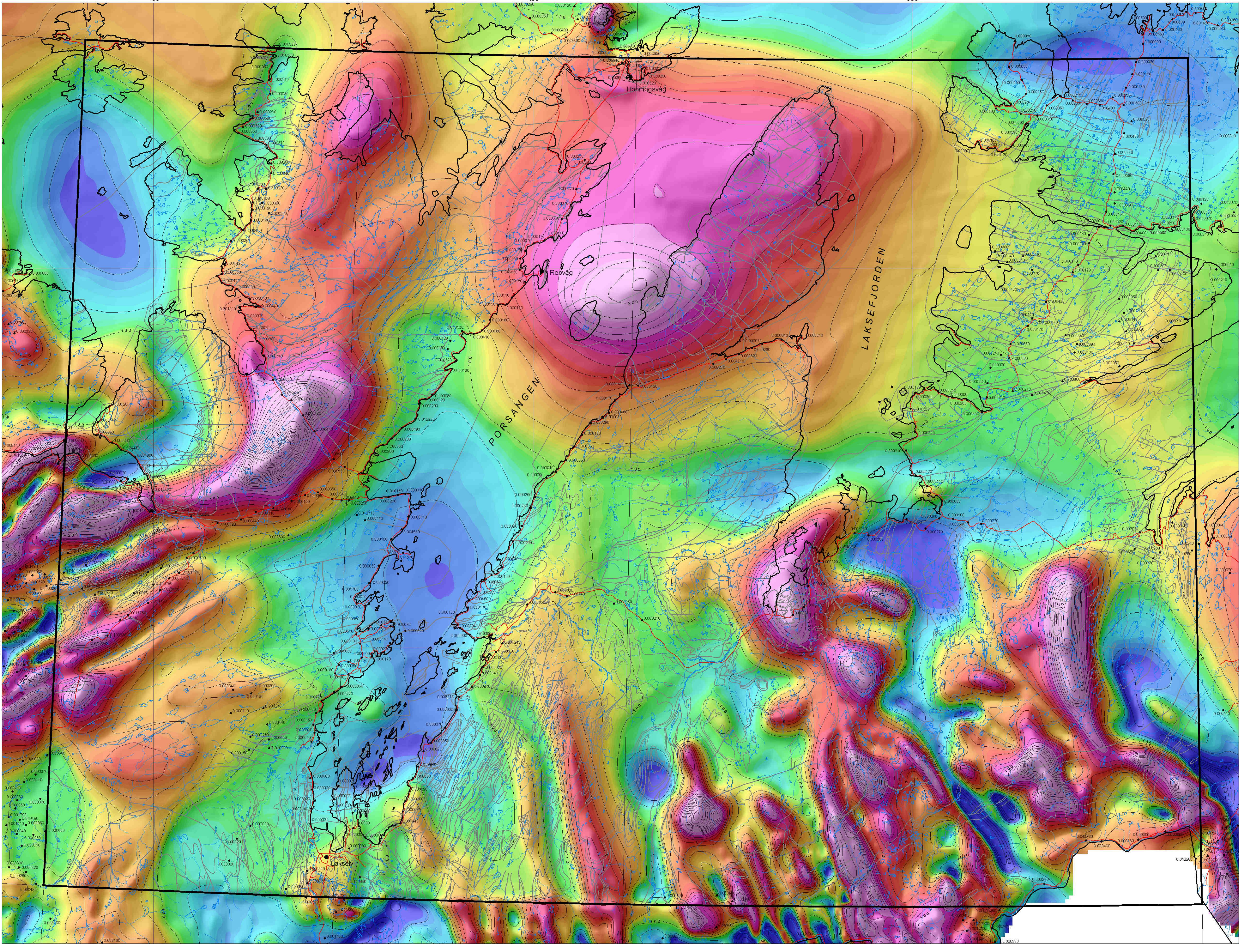
TYNNEANOMALIKART Terrain-corrected magnetic anomalies
