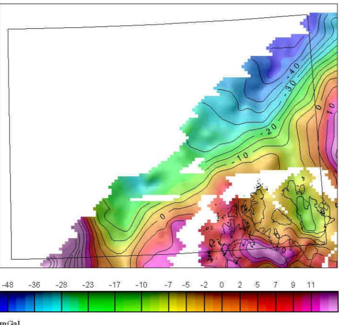
GRAVIMETRISK RESIDUALKART GRAVITY RESIDUAL MAP
