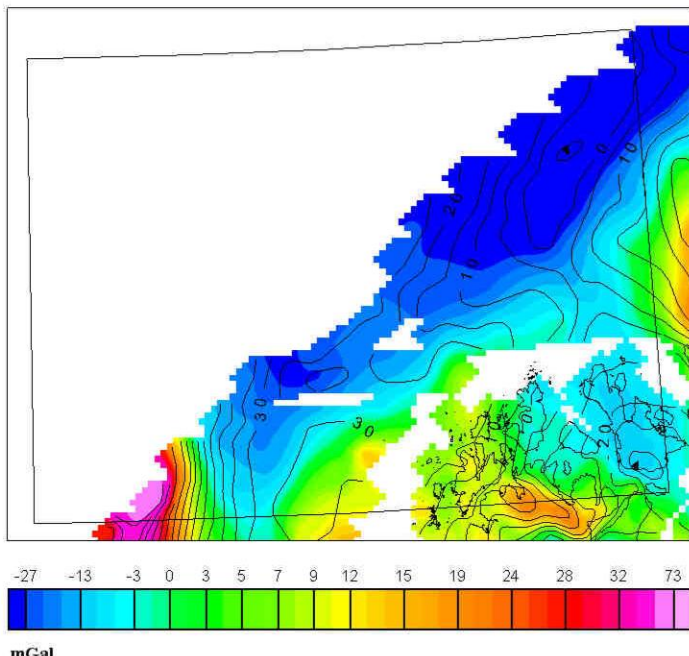
TYSNGEANOMALIKART Terrenghøitrigerte bouguer-anomalier GRAVITY ANOMALY MAP Terrain-corrected bouguer anomalies
