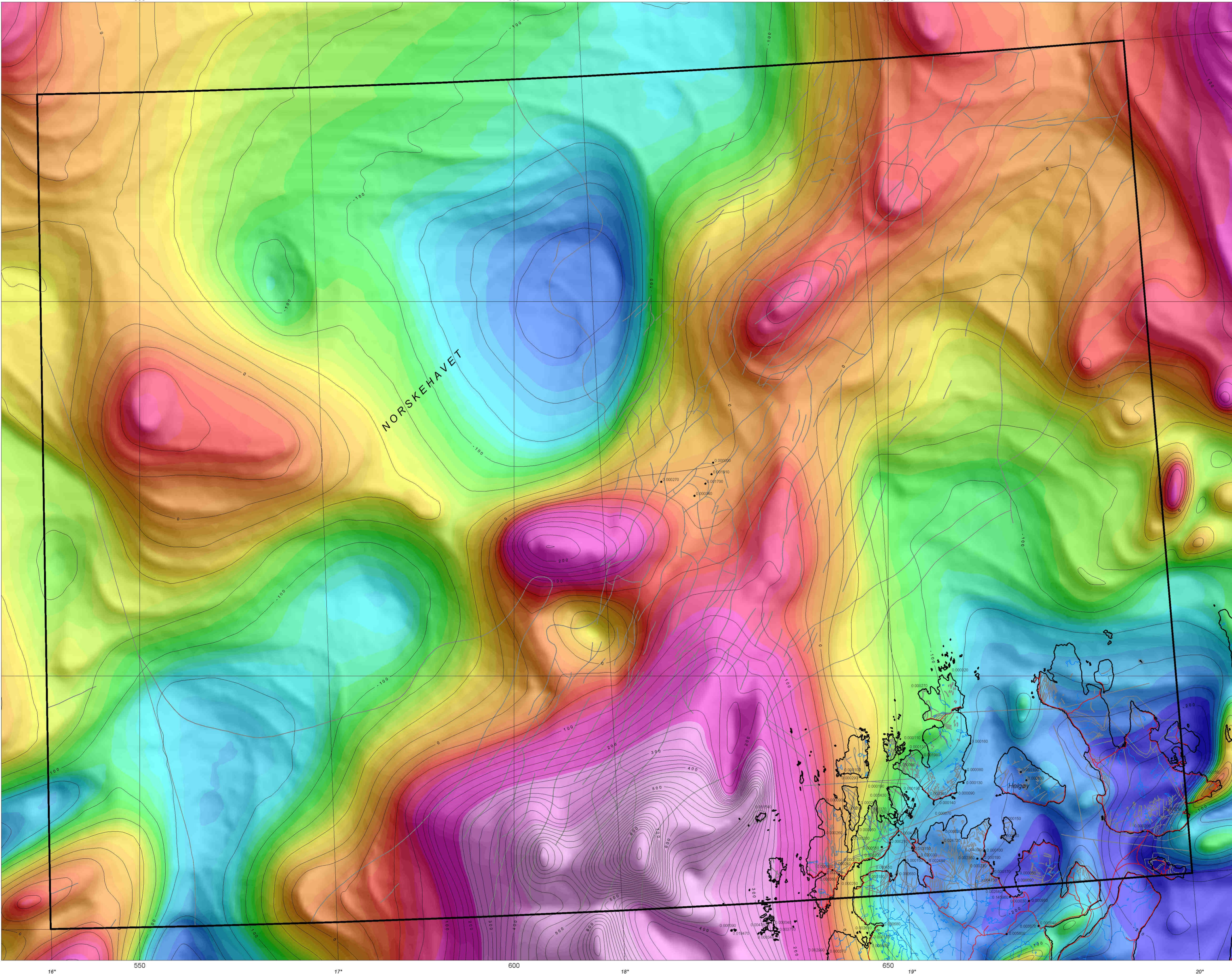
TYSNGEANOMALIKART Terrenghøitrigerte bouguer-anomalier GRAVITY ANOMALY MAP Terrain-corrected bouguer anomalies
