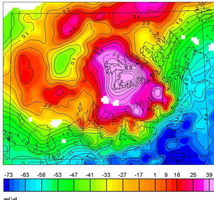
TYNGDEANOMALIKART Terrestrial gravity anomalies
