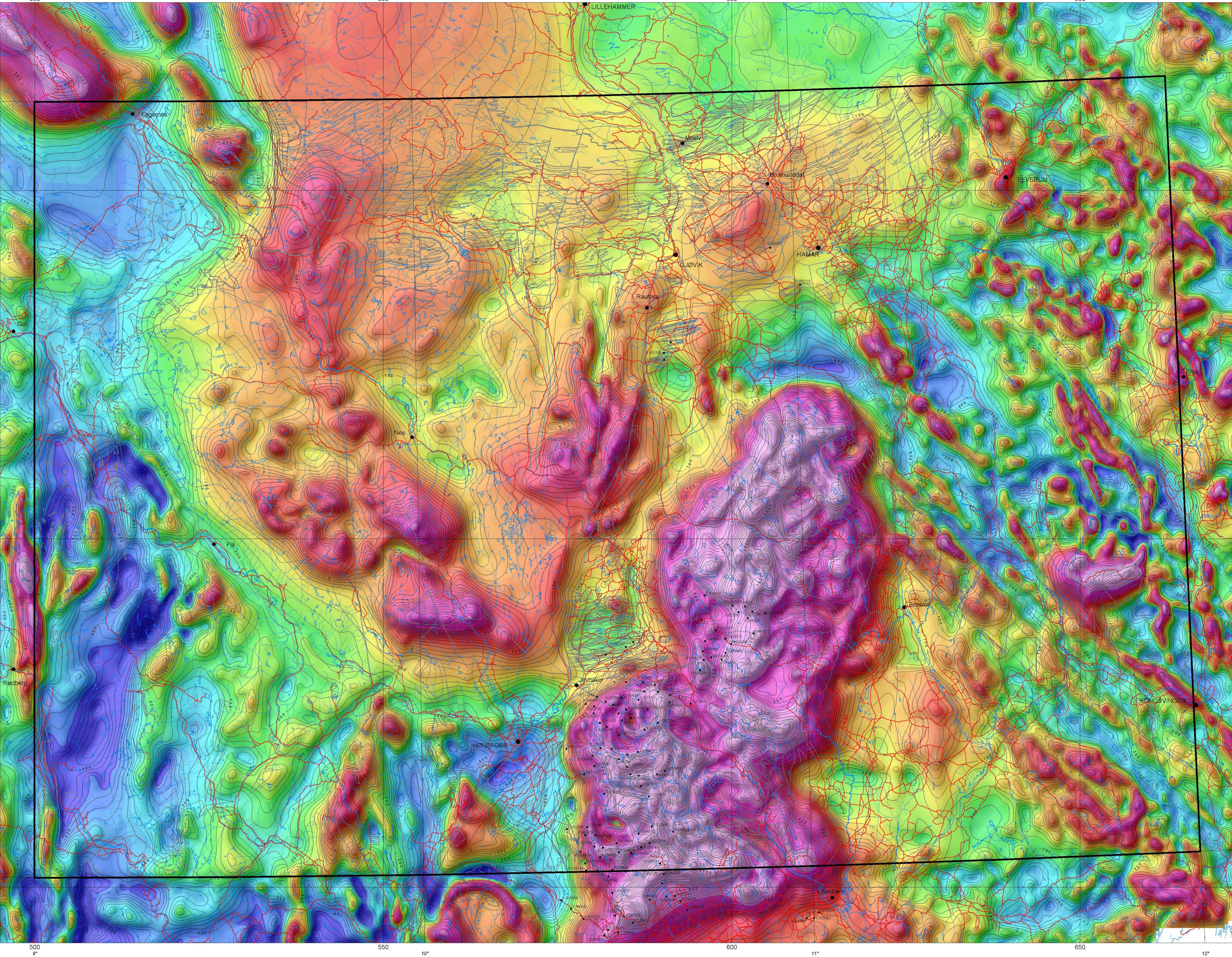
TYNGDEANOMALIKART Terrengkorrigerte langper anomaler GRAVITY ANOMALY MAP Terrain-corrected longwave anomalies
