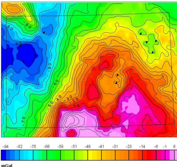
TYNGDEANOMALIKART Terrengkorrigerte langper anomaler GRAVITY ANOMALY MAP Terrain-corrected longwave anomalies
