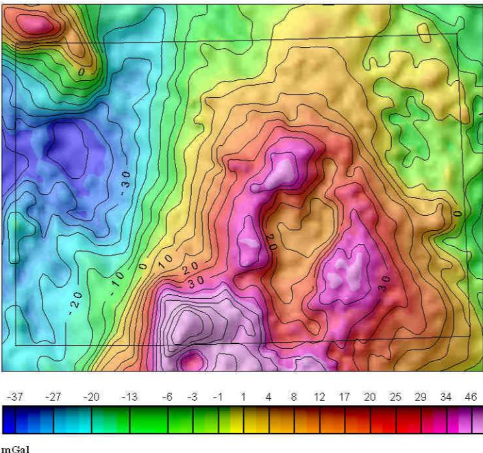
GRAVIMETRISK RESIDUALKART GRAVITY RESIDUAL MAP
