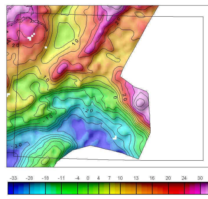
GRAVITY RESIDUAL MAP
