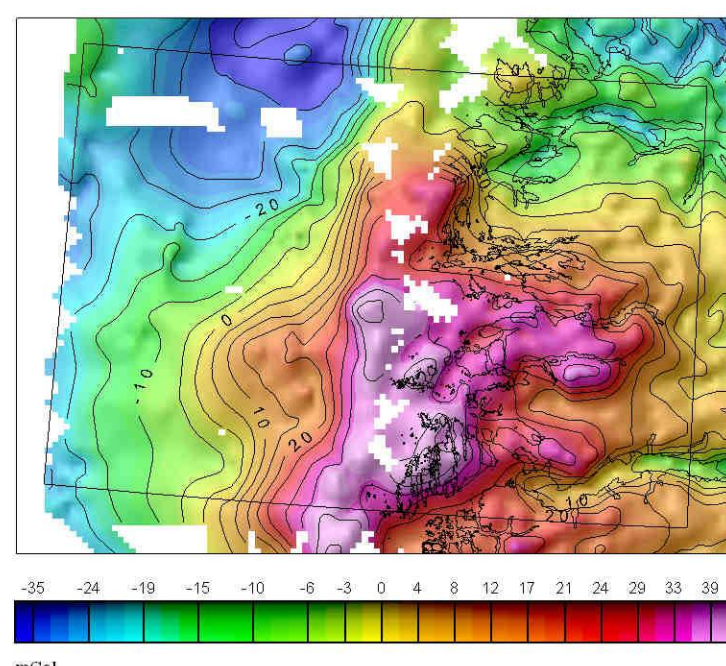
GRAVITY RESIDUAL MAP
