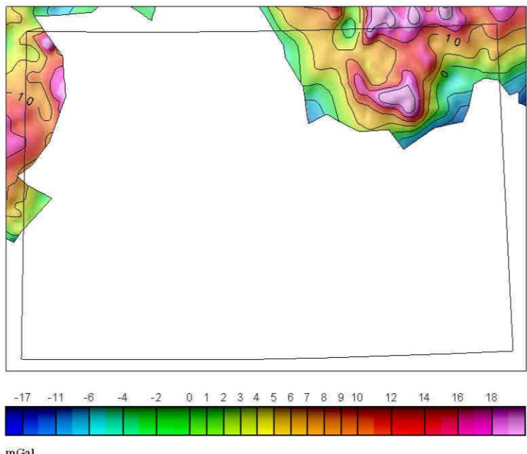
GRAVIMETRISK RESIDUALKART GRAVITY RESIDUAL MAP
