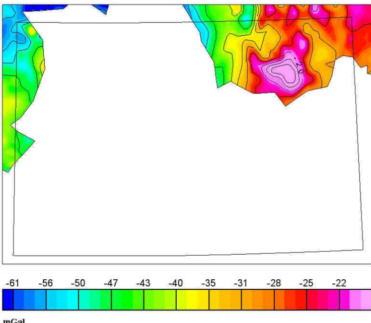
TYNGDEANOMALIKART Terrengkorrigerte langsomme anomalier GRAVITY ANOMALY MAP Terrain-corrected longwave anomalies
