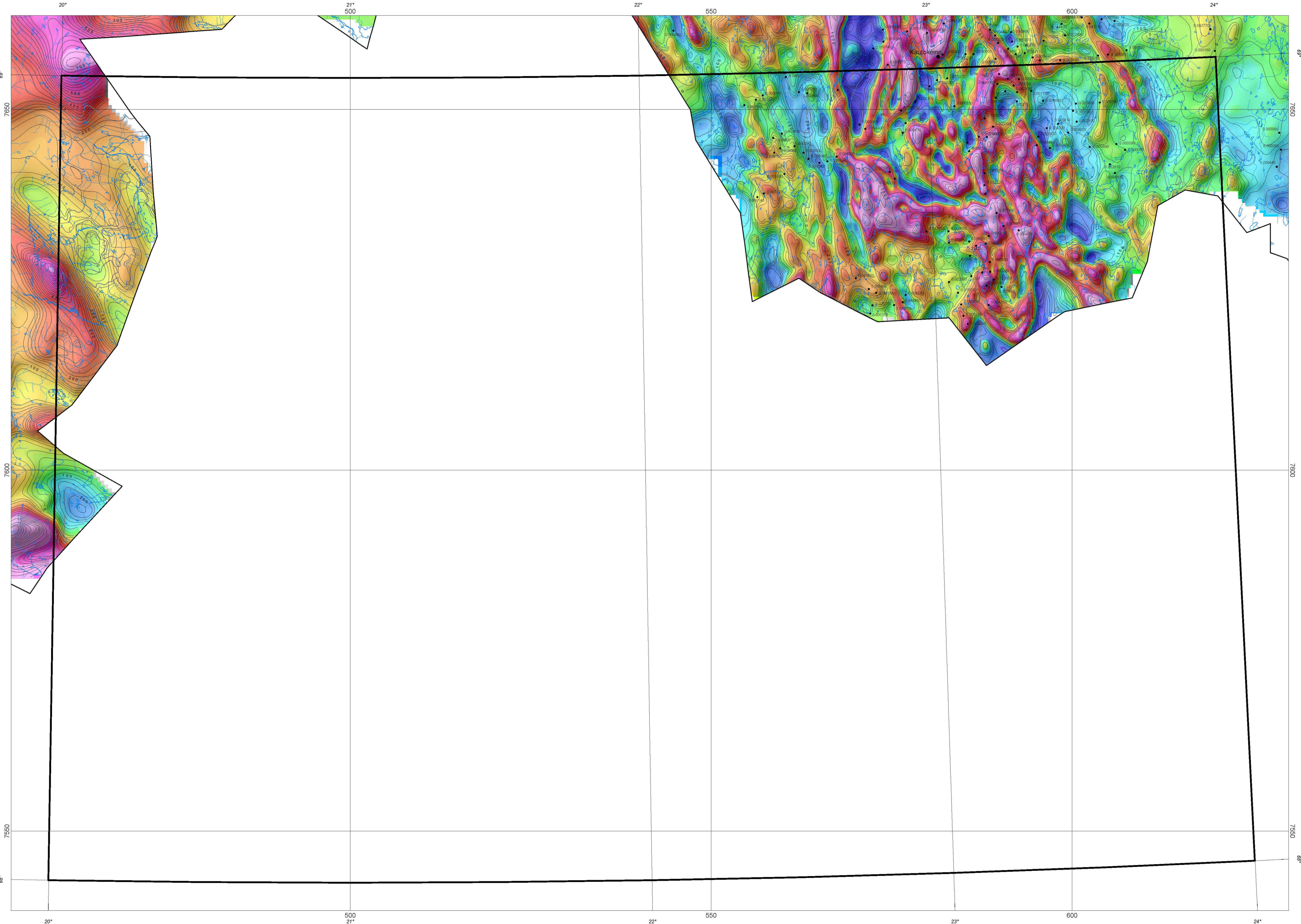
TYNGDEANOMALIKART Terrengkorrigerte langsomme anomalier GRAVITY ANOMALY MAP Terrain-corrected longwave anomalies
