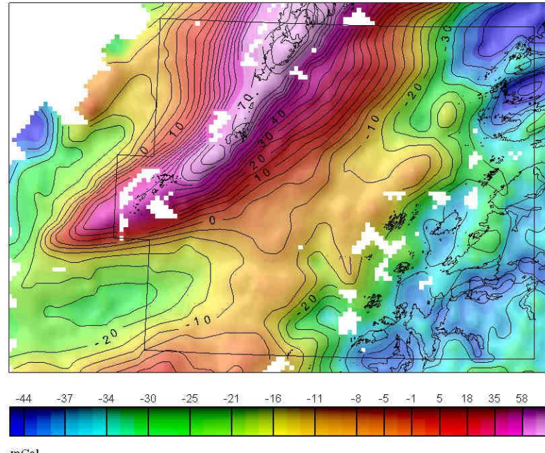
GRAVIMETRISK RESIDUALKART Magnetfeltet referert til DGRF 1965.0 GRAVITY RESIDUAL MAP Magnetic field referred to DGRF 1965.0
