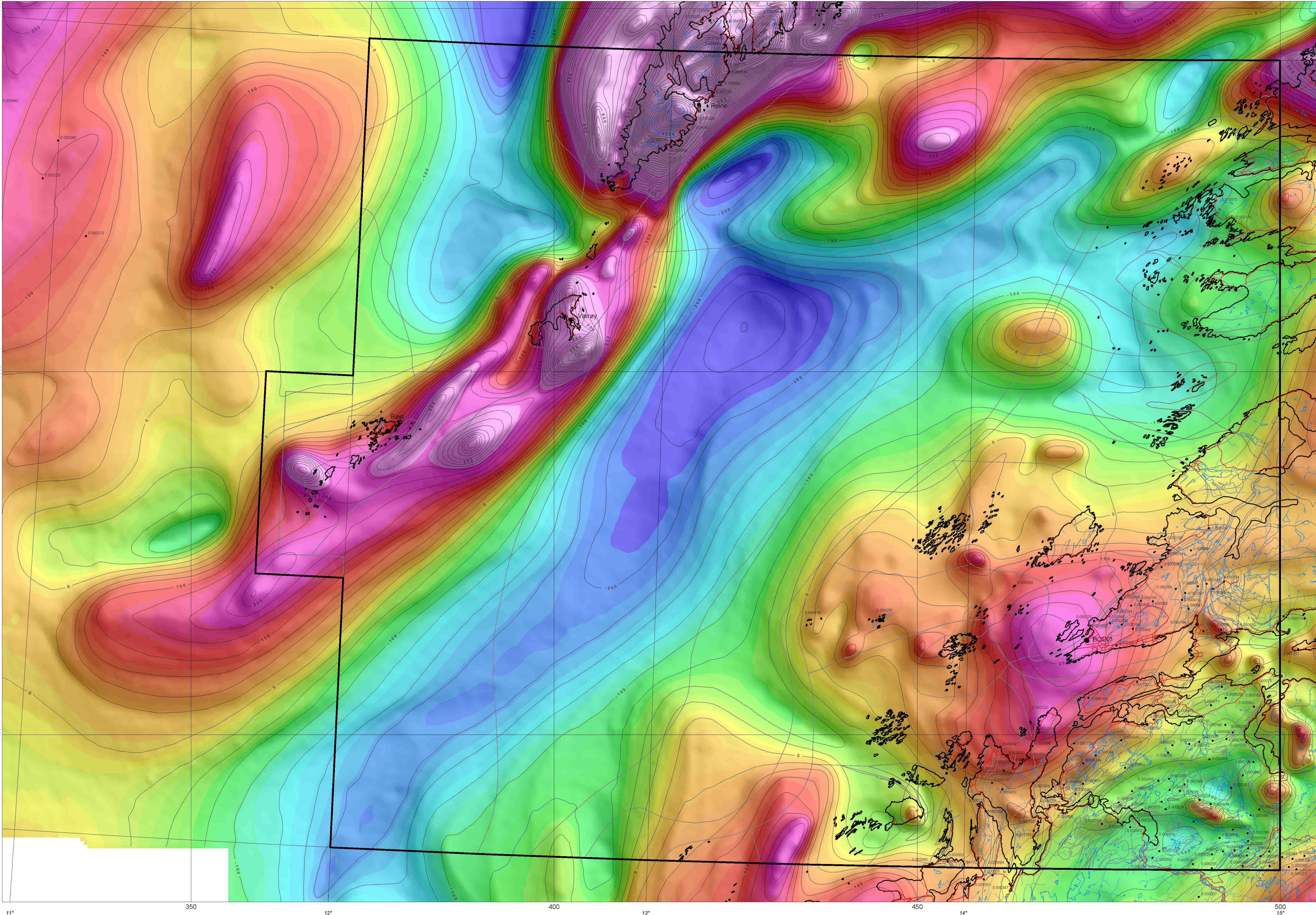
TYNGDEANOMALIKART Tyngdekompenserte langsgående anomalier GRAVITY ANOMALY MAP Terrain-corrected long-range anomalies
