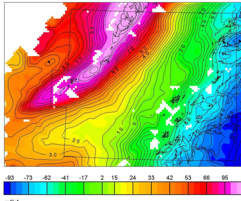
TYNGDEANOMALIKART Tyngdekompenserte langsgående anomalier GRAVITY ANOMALY MAP Terrain-corrected long-range anomalies
