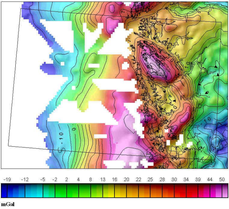
GRAVIMETRISK RESIDUALKART Magnetfeltet referert til GMR 1965.0 GRAVITY RESIDUAL MAP Magnetic field referred to DGRF 1965.0
