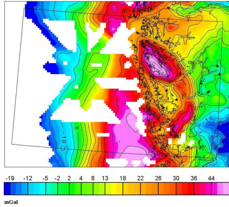
FYNGERANOMALIKART Terrain-corrected bouguer anomalies GRAVITY ANOMALY MAP Terrain-corrected bouguer anomalies
