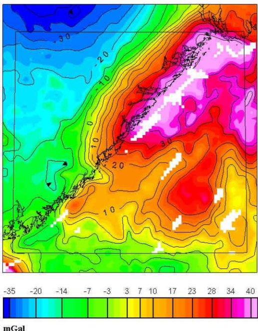
TYNGDEANOMALIKART Terrengkorrigerte bouguer anomalier GRAVITY ANOMALY MAP Terrain-corrected bouguer anomalies
