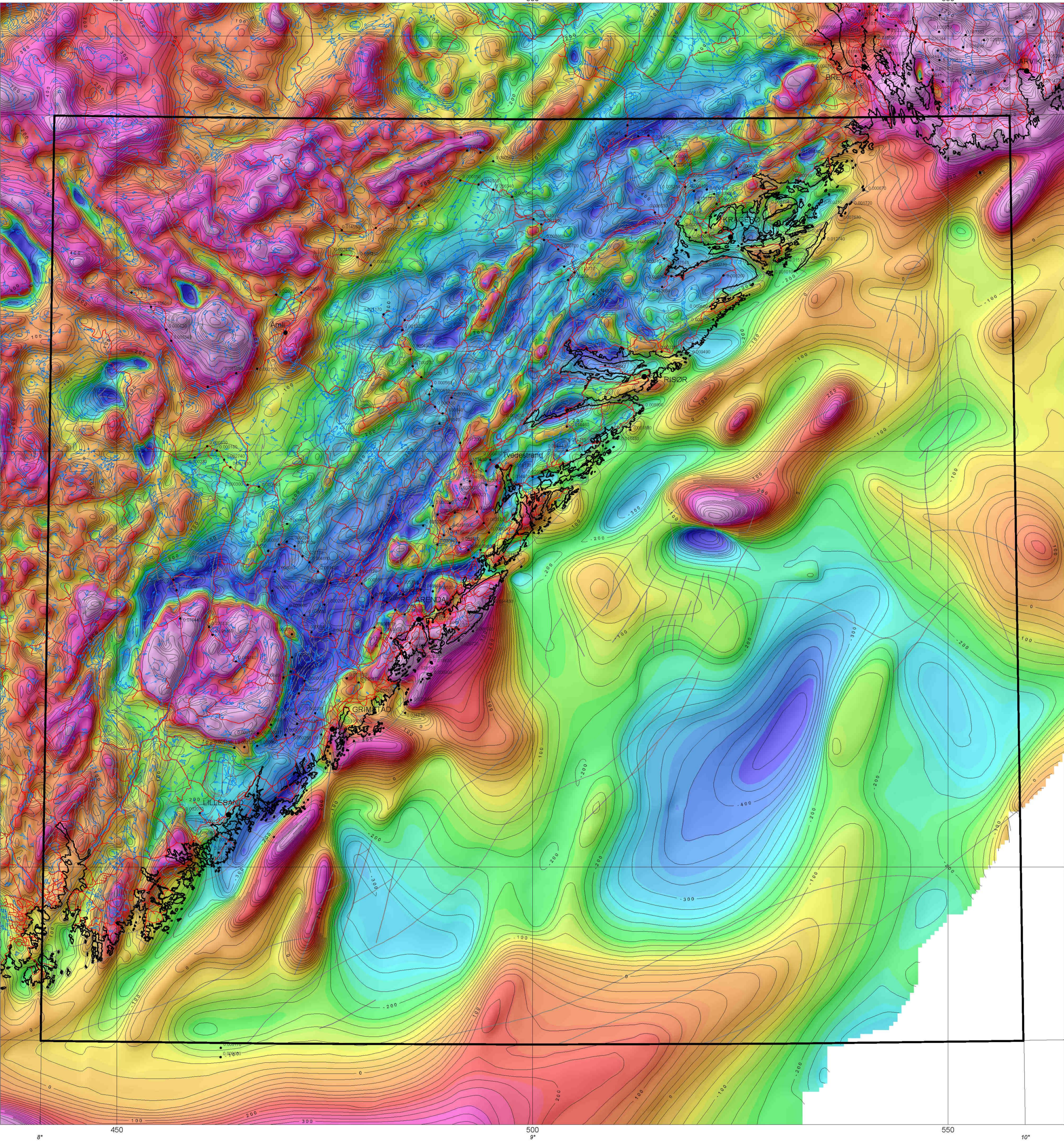
TYNGDEANOMALIKART Terrengkorrigerte bouguer anomalier GRAVITY ANOMALY MAP Terrain-corrected bouguer anomalies
