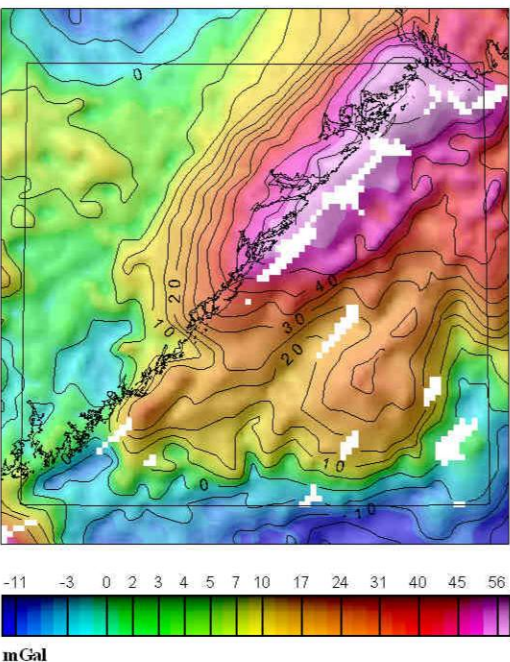
GRAVIMETRISK RESIDUALKART Magnetfeltet referert til DGRF 1965.0 GRAVITY RESIDUAL MAP Magnetic field referred to DGRF 1965.0
