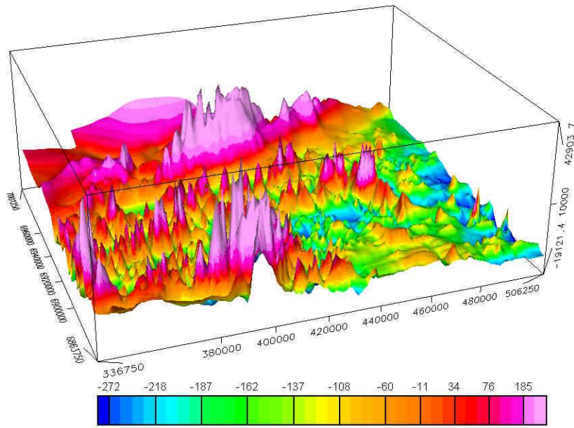
AEROMAGNETISK 3D ANOMALIKART Magnetic field referred to DGRF 1965.0
