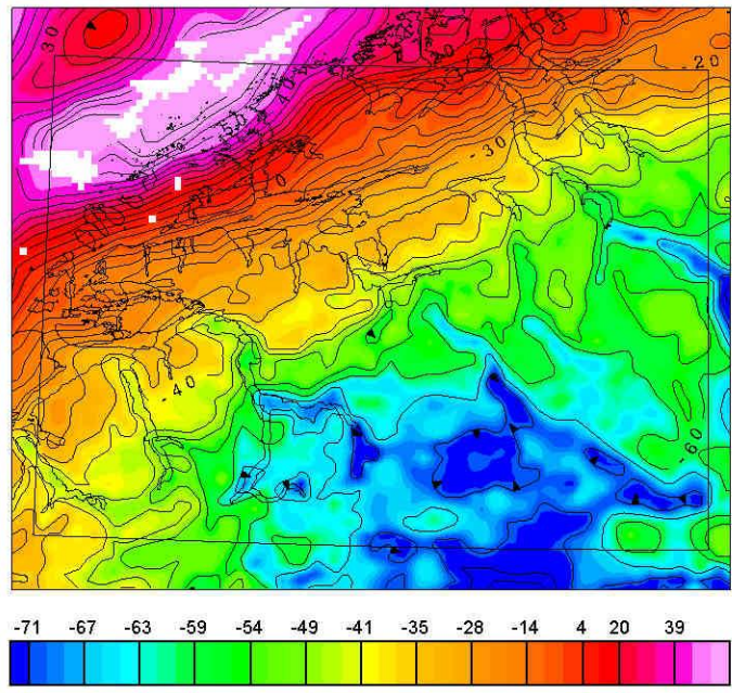
TYNGDEANOMALIKART Terrain-corrected magnetic anomalies
