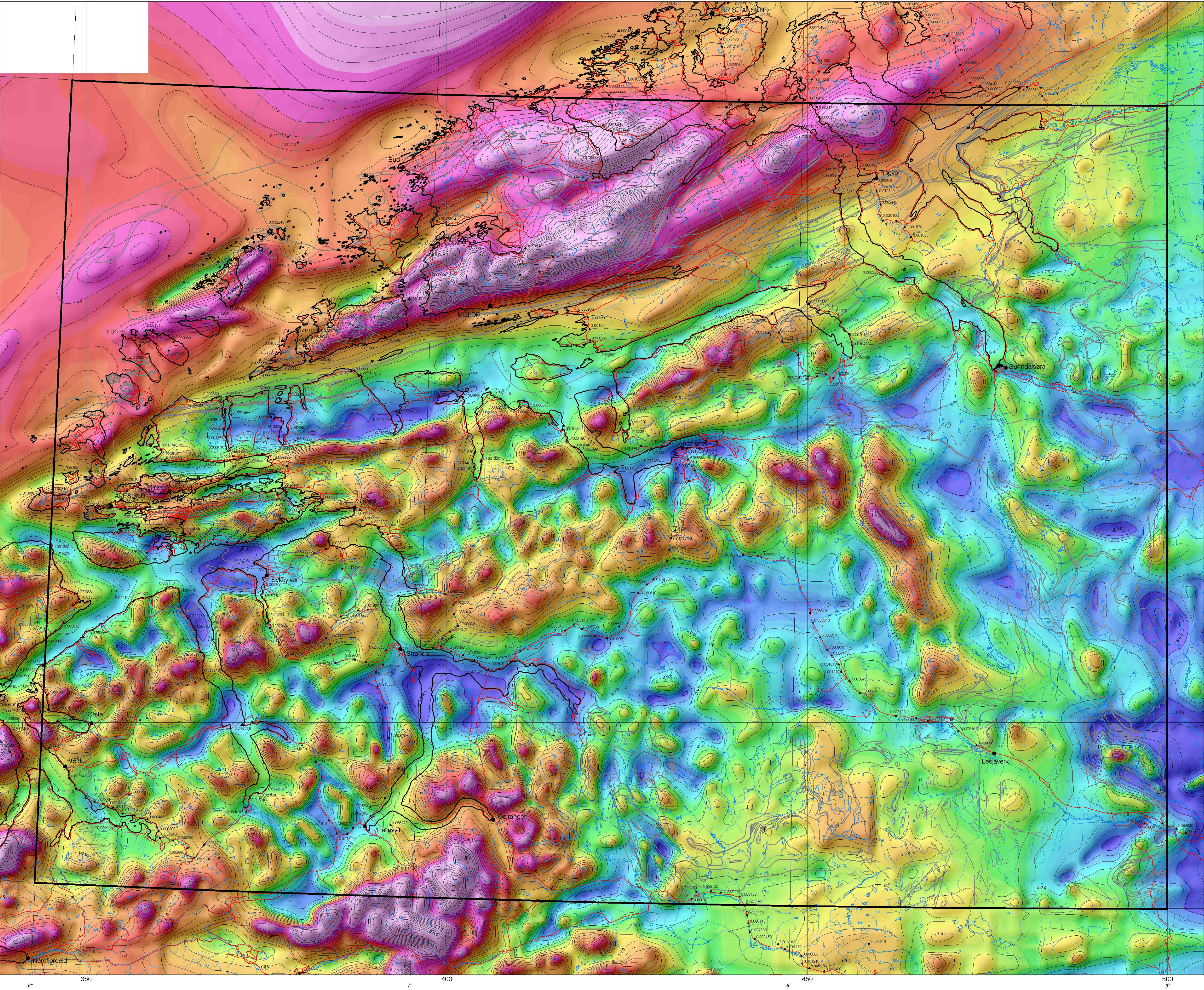
TYNGDEANOMALIKART Terrain-corrected magnetic anomalies
