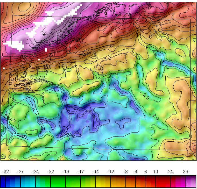
GRAVITETRISK RESIDUALKART Gravitv residual map
